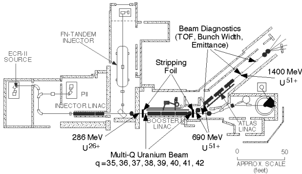
Figure 3: Layout of ATLAS linac.
