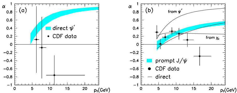
Figure 6: Polarization variable \alpha vs. p_T for (a) direct \psi' and (b) prompt J/\psi compared to CDF data. 39 100% transverse polarization corresponds to \alpha = 1 .
