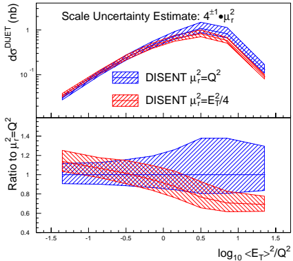
Figure 2: NLO QCD scale uncertainty estimates for the DIS dijet cross section as obtained with the DISENT 7 program. 3
