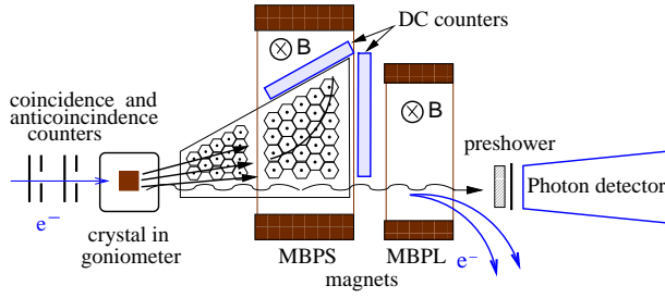
Figure 1: Experimental set-up
