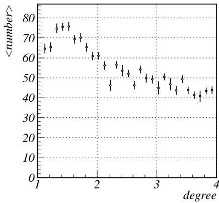
Figure 4: Rocking curve measured with number of wires in DC for the hybrid target.
