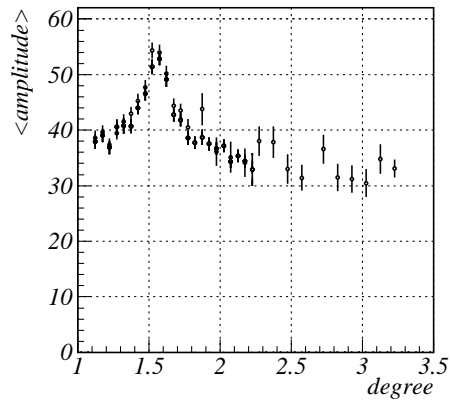
Figure 2: Rocking curve measured on preshower for the hybrid target.
