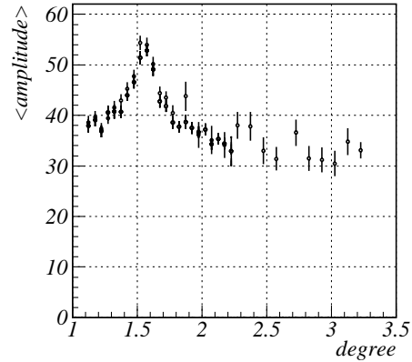
Figure 2: Rocking curve measured on preshower for the hybrid target.
