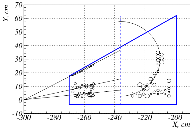
Figure 5: Typical event for the hybrid target. Field 0.4T
