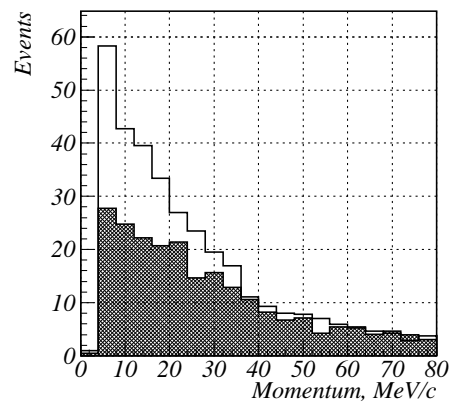
Figure 6: Positron momentum distribution measured by DC with hybrid target. Field 1 kGauss. Incident energy is 10 GeV. The unfilled histogram represent the oriented crystal, dark one — the target in random position.
