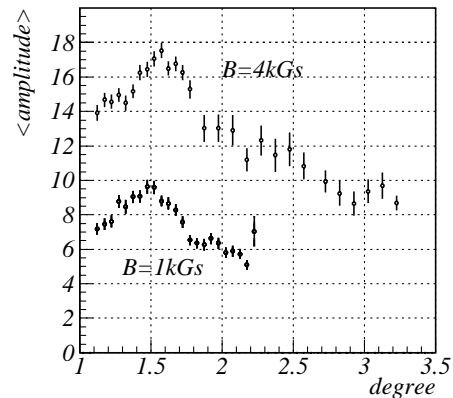
Figure 3: Rocking curves measured on DC counter 1 for the hybrid target with two values of the magnetic field.
