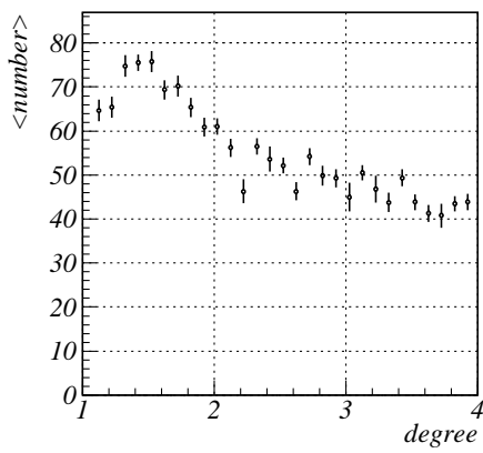
Figure 4: Rocking curve measured with number of wires in DC for the hybrid target.
