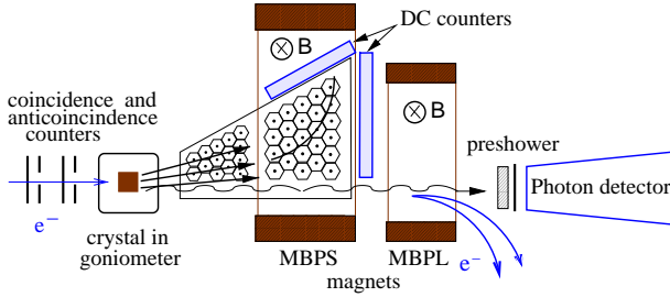
Figure 1: Experimental set-up
