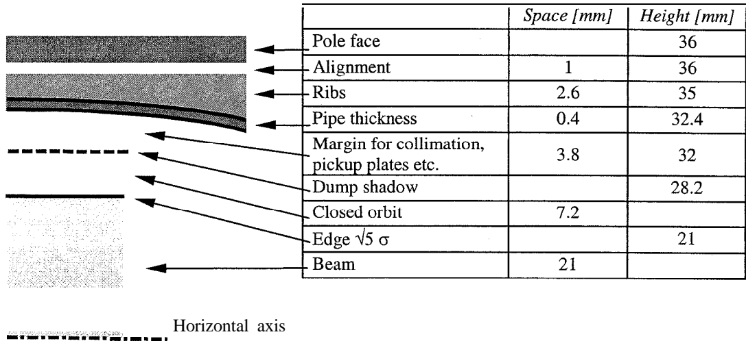
Fig. 2 Vertical half aperture of synchrotron dipoles.
