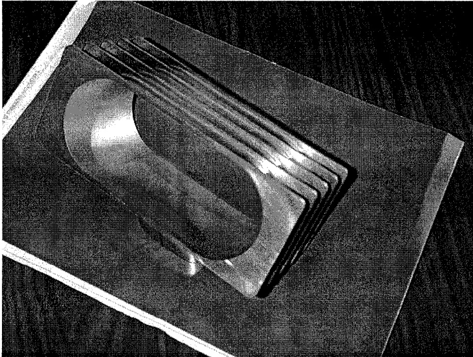
Fig. 6 The second thin chamber prototype realised in Frascati.
