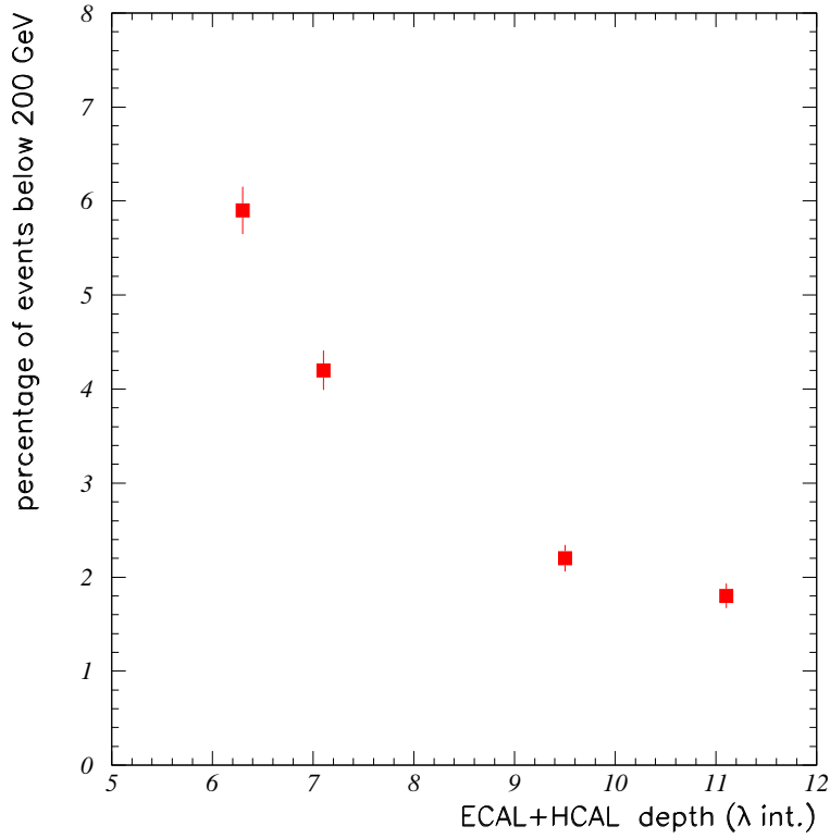
Fig. 34. H2(1996) data, B = 3 Tesla: the fraction of 300 \text{ GeV}/c pions with reconstructed energy less than 200 \text{ GeV} (approximately 3 \sigma below the mean, or 100 \text{ GeV} of missing energy) versus total absorber depth. The total \lambda_{INT} includes the contribution of ECAL.
