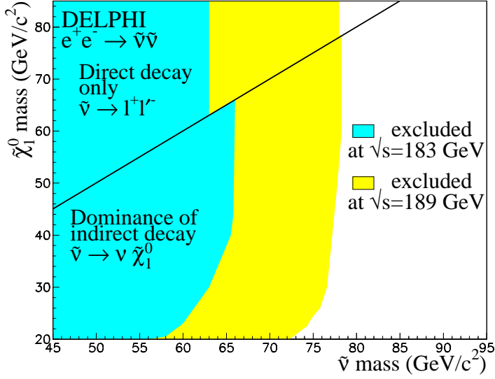
Figure 5: Excluded region at 95% C.L. in m_{\tilde{\chi}^0} , m_{\tilde{\nu}} parameter space by \tilde{\nu} pair production for direct and indirect decays. The dark grey area shows the part excluded by the searches at 183 GeV, the light grey area the one excluded by the present analysis.
