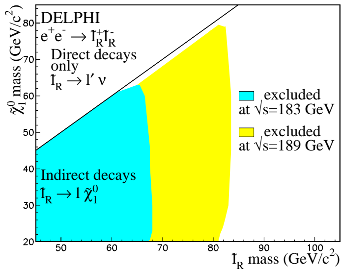
Figure 6: Charged slepton indirect decay: excluded region at 95% C.L. in m_{\tilde{\chi}^0_1} , m_{\tilde{\ell}_R} parameter space by \tilde{\ell}_R pair production. The dark grey area shows the part excluded by the searches at 183 GeV, the light grey area the one excluded by the present searches at 189 GeV.
