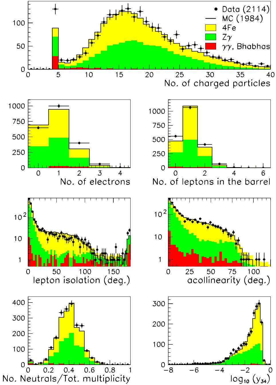
Figure 1: Distributions, after the preselection applied for the \lambda_{133} analyses, of the number of charged particles, the number of well identified electrons in the event, the number of identified leptons with a polar angle between 40^\circ and 140^\circ , the lepton isolation angle, the acollinearity, the ratio of the number of neutral particles to the total event multiplicity, and the \log_{10}(y_{34}) . The black dots show the real data distributions, and the shaded histograms the expected background from Standard Model processes.
