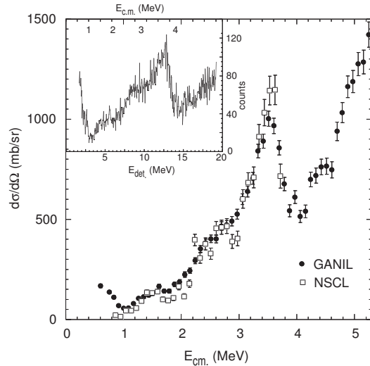
FIG. 3. The excitation function of ^{11}\text{N} is shown after background subtraction and transformation to the c.m. system. The filled black circles represent the GANIL data, and the white squares show the result of the MSU experiment. The inset shows the raw data in the lab. system. The upper scale in the inset is a rough calibration to c.m. energy, shown for comparison, while the lower scale is the detected proton energy.
