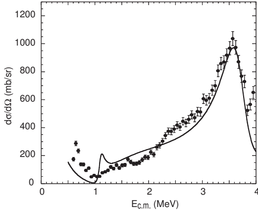
FIG. 5. A typical fit of the experimental data when the 1/2^- state is assumed to be the ground state of ^{11}\text{N} . It is evident that the excitation function is not well described. Putting the p state this low makes it too narrow, at the same time as the s state becomes very broad since it is now well above the Coulomb barrier.
