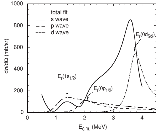
FIG. 6. The partial waves s_{1/2} , p_{1/2} and d_{5/2} together with the total calculated excitation function for the best fit to the experimental data (Table I:c).
