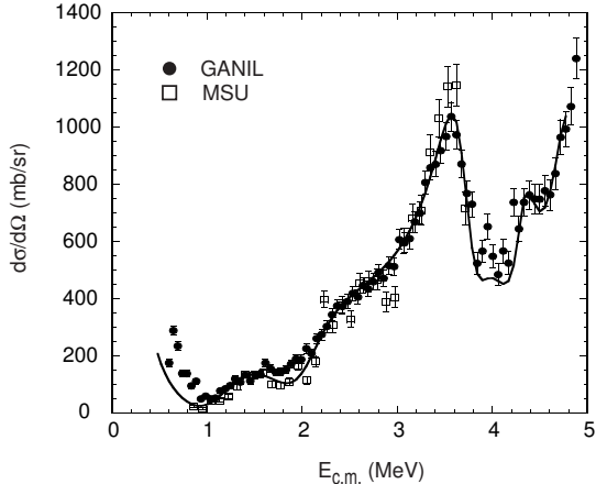
FIG. 9. The fit of the potential model with added resonances. The full drawn curve includes the two known resonances in ^{11}\text{Be} plus a broad 3/2^+ level around 4 MeV and a high-spin state at 5.4 MeV, which gives a good description of the full excitation function up to 4.7 MeV. Especially it should be noted that the theoretical curve now better reproduces the data at 1.6-2.0 MeV.
