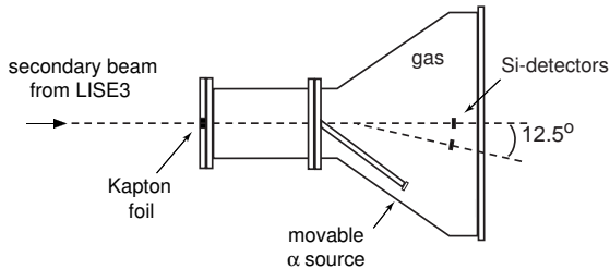
FIG. 1. A schematic view of the scattering chamber and Si-detectors. The 12.5^\circ detector has this angle to the middle of the chamber. The interaction position and the corresponding angle is calculated for each event when analyzing the data.
