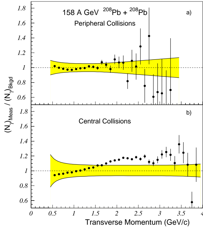
FIG. 31. The \gamma_{\text{Meas}}/\gamma_{\text{Bkgd}} ratio as a function of transverse momentum for peripheral (part a)) and central (part b)) 158 A GeV ^{208}\text{Pb}+^{208}\text{Pb} collisions for the sum of 1995 and 1996 magnet on data sets. The narrow shower photon identification criterion has been used. The errors on the data points indicate the statistical errors only. The p_T -dependent systematical errors are indicated by the shaded bands ( \equiv 1_{-\sigma_U}^{+\sigma_L} ). (Note: Upper and lower errors are inverted for display purposes.)
