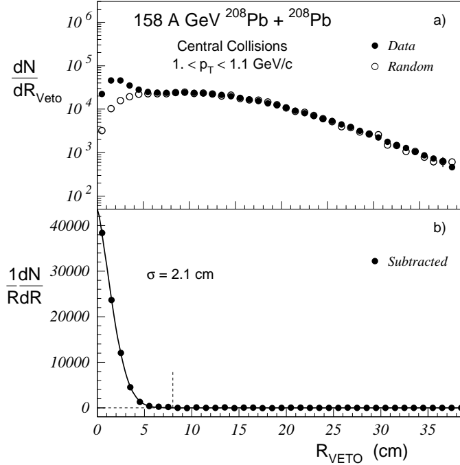
FIG. 7. The distribution of distances, R_{Veto} , to the nearest CPV hit from a shower particle in the lead-glass for central events. In part a) the distribution for real events is shown by the solid circles. The distribution for randomly vetoed hits is shown by the open circles. The random veto distribution is obtained using test GEANT showers inserted into real events. The true veto radius distribution after subtraction of the random veto distribution is shown in part b).
