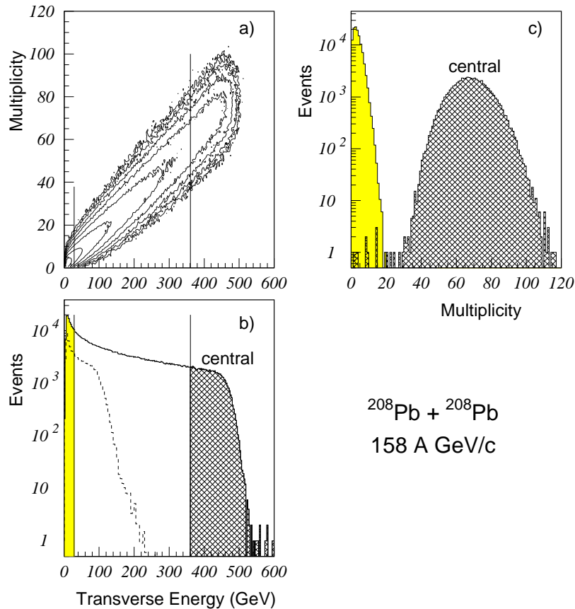
FIG. 5. The correlation between the number of showers observed in the lead-glass detector and the measured transverse energy for 158 A GeV ^{208}\text{Pb}+^{208}\text{Pb} collisions for a sample of the 1995 magnet on data. Part b) shows the projection onto the transverse energy axis with the shaded regions indicating the peripheral and central event class selections used for the present analysis. The distribution is uncorrected for the empty target contribution which is shown by the dashed histogram with arbitrary relative normalization. Part c) shows the projection onto the lead-glass multiplicity axis for the selected events.
