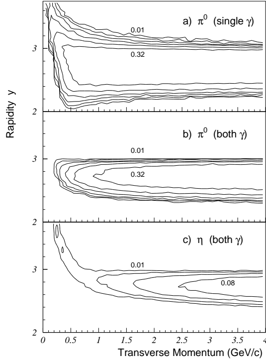
FIG. 2. The acceptance of the WA98 photon spectrometer in parent particle rapidity versus transverse momentum for a) single photons from \pi^0 decay and for photon-pairs from b) \pi^0 decay or c) \eta decay with a 750 MeV photon energy threshold. The contours show the fraction of full phi acceptance in steps of factors of two.
