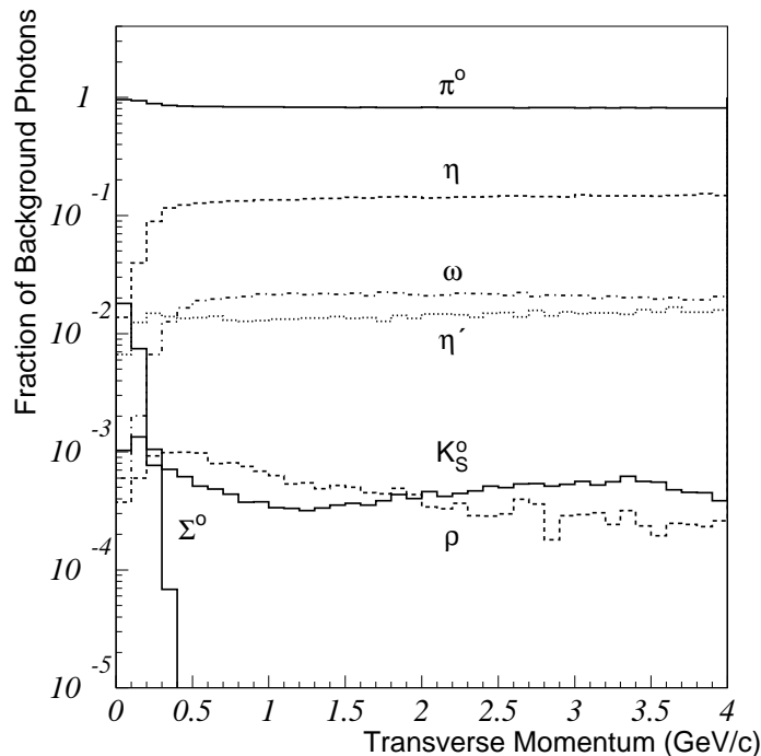
FIG. 28. The calculated fraction of all background inclusive photons from various radiative decay sources is shown as a function of the transverse momentum for central 158 A GeV ^{208}\text{Pb}+^{208}\text{Pb} collisions.
