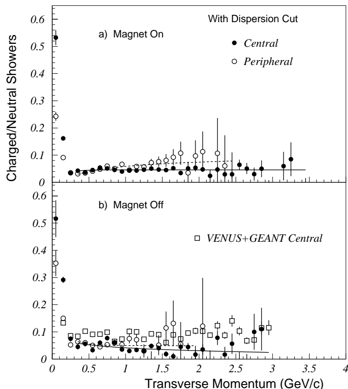
FIG. 11. The measured ratio of charged to neutral showers in the lead-glass detector for peripheral (open circles) and central (solid circles) 158 A GeV ^{208}\text{Pb}+^{208}\text{Pb} collisions as a function of the transverse momentum of the cluster. The results are shown for clusters which pass a photon-like dispersion cut for a) magnet on and b) magnet off. The data have been corrected for photon conversions and the CPV efficiency. The lines are fitted curves.
