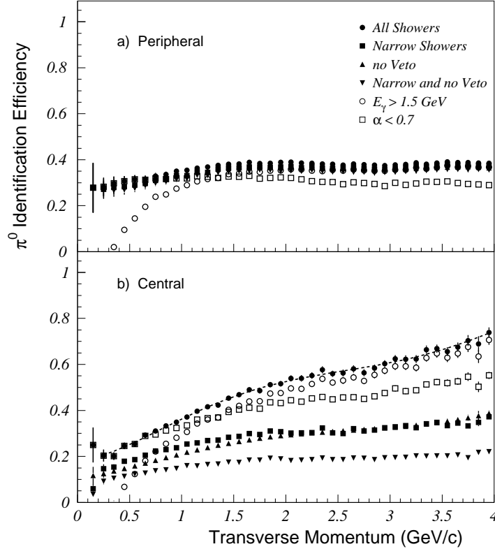
FIG. 22. The \pi^0 identification efficiency including effects of resolution, shower overlap, and excluded lead-glass modules. The \pi^0 identification efficiency is shown as a function of transverse momentum for a) peripheral and b) central 158 A GeV ^{208}\text{Pb}+^{208}\text{Pb} collisions. A 750 MeV shower energy threshold has been applied. The efficiency is shown for the 1996 magnet on data for the following criteria: all showers (solid circles), showers satisfying a dispersion cut (solid squares), all showers with no associated hit in the CPV (solid triangles), all showers satisfying a dispersion cut with no associated hit in the CPV (inverted solid triangles), all showers but with shower energy threshold increased to 1.5 GeV/c (open circles), and all showers with the requirement that the shower-pair energy asymmetry is less than 0.7 (open squares). An example of the fitted parameterization of the efficiency is shown by the dashed curve in part b) for the criterion of using all showers.
