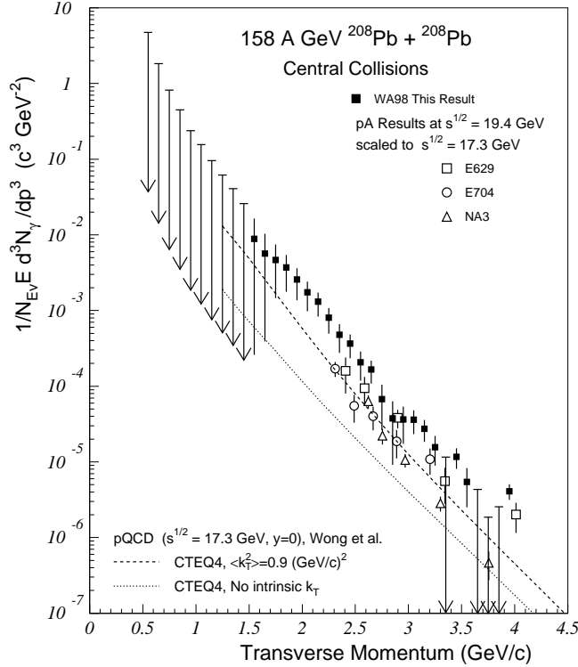
FIG. 32. The invariant direct photon multiplicity for central 158 A GeV ^{208}\text{Pb}+^{208}\text{Pb} collisions. The error bars indicate the combined statistical and systematical errors. Data points with downward arrows indicate unbounded 90% CL upper limits. Results of several direct photon measurements for proton-induced reactions have been scaled to central 158 A GeV ^{208}\text{Pb}+^{208}\text{Pb} collisions for comparison. The calculation is described in the text.
