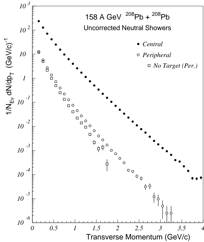
FIG. 12. The multiplicity of all neutral showers as a function of transverse momentum for peripheral (open circles) and central (solid circles) 158 A GeV ^{208}\text{Pb}+^{208}\text{Pb} collisions. The results are the sum of 1995 and 1996 magnet on data sets. Results are also shown (open squares) for peripheral event selection for runs with no target. The spectra have not been corrected for efficiency or acceptance. They are used as the first iteration in the iterative efficiency correction.
