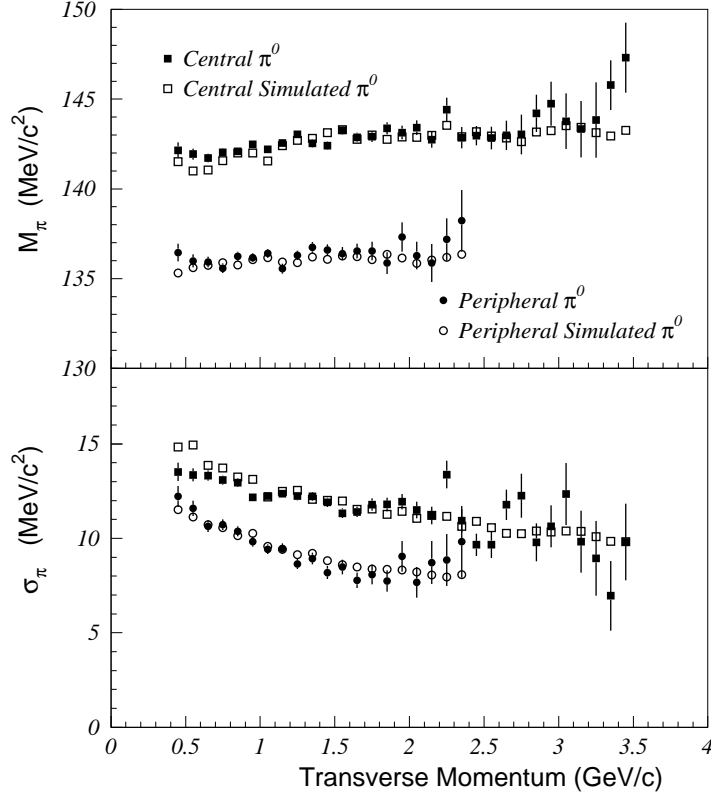
FIG. 21. The \pi^0 mass peak position and width, \sigma , resulting from a gaussian fit to the two-photon invariant mass distribution is shown as a function of the transverse momentum in the upper and lower portions of the figure, respectively. The solid symbols show results for real \pi^0 's while the open points show the results for simulated \pi^0 's superimposed on real events. Results are shown for peripheral (circles) and central (squares) 158 A GeV ^{208}\text{Pb}+^{208}\text{Pb} collisions using all shower candidates. The same fit region is used for the real and simulated data.
