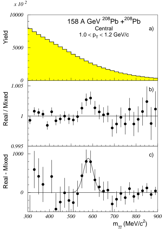
FIG. 24. The two-photon invariant mass distribution for central events in the \eta mass region with photon pair transverse momentum 1.0 < p_T < 1.2 \text{ GeV}/c . Part a) shows the invariant mass distribution for all shower pairs for real events (solid histogram) and mixed events (filled histogram). Part b) shows the ratio of real and mixed event mass distributions. Part c) shows the real invariant mass distribution after subtracting the normalized mixed event distribution.
