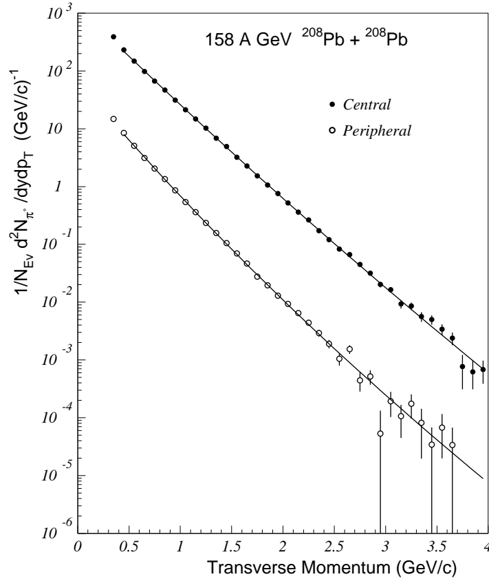
FIG. 26. The \pi^0 transverse momentum distribution for peripheral (open circles) and central (solid circles) 158 A GeV ^{208}\text{Pb}+^{208}\text{Pb} collisions for the sum of 1995 and 1996 magnet on data sets. The narrow shower photon identification criterion has been used. The data have been corrected for efficiency and acceptance. Only statistical errors are shown. The solid curves show the fit results described in the text.
