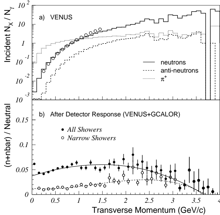
FIG. 13. In part a) the ratio of neutrons (solid line), anti-neutrons (dashed line), and \pi^+ (dotted line) to photons into the LEDA acceptance is shown as a function of the transverse momentum. The results are predictions of the VENUS 4.12 event generator for central 158 A GeV ^{208}\text{Pb}+^{208}\text{Pb} collisions. The open points are described in the text. In part b) the ratio of neutrons plus anti-neutrons to neutral ( n + \bar{n} + \gamma ) is shown after the effects of the lead-glass detector response calculated with GEANT. Results are shown after application of shower identification criteria of using all showers (solid circles) or narrow showers (open circles). The curves are fit results.
