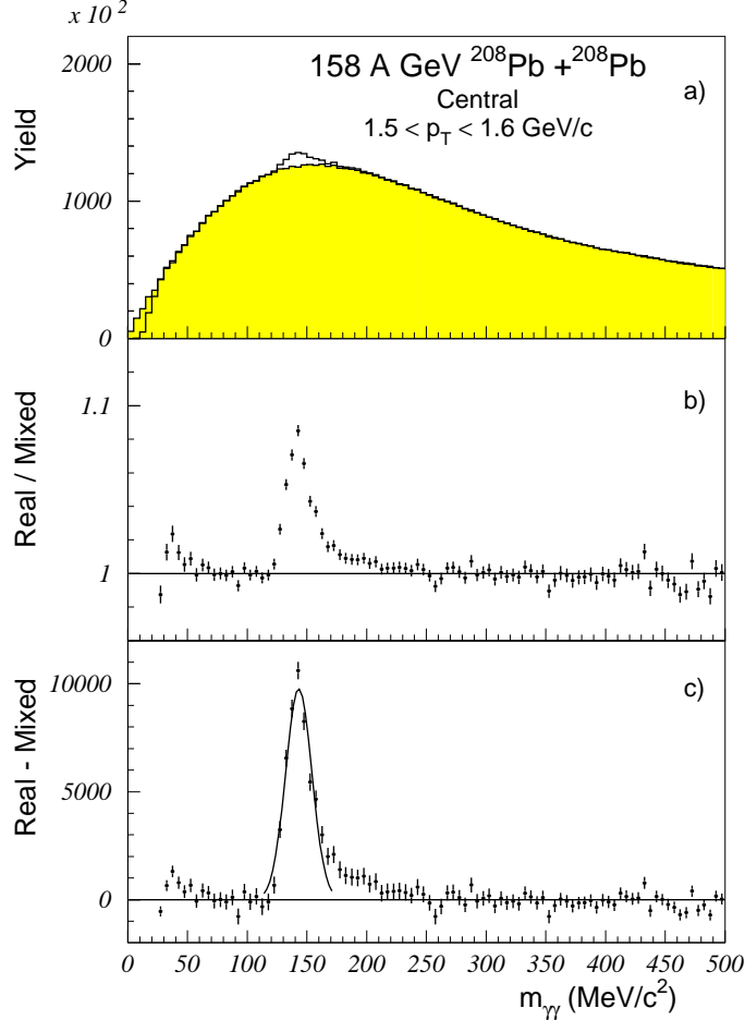
FIG. 19. The two-photon invariant mass distribution for central events in the \pi^0 mass region with pair transverse momentum 1.5 < p_T < 1.6 \text{ GeV}/c . Results are shown for the 1995 magnet on data sample. Part a) shows the invariant mass distribution for all shower pairs for real events (solid histogram) and mixed events (filled histogram). Part b) shows the ratio of real and mixed event mass distributions. Part c) shows the real invariant mass distribution after subtracting the normalized mixed event distribution.
