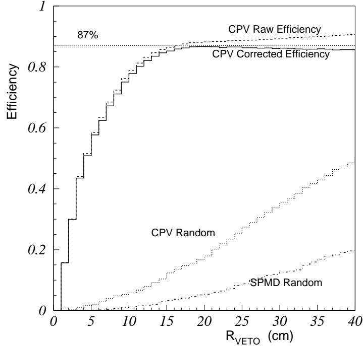
FIG. 9. The efficiency of the charged particle veto as a function of veto radius. The results are obtained from magnetic field off peripheral data. The dashed curve shows the probability that a hit in the CPV is found within a distance R_{Veto} of a charged hit in the lead-glass. The lead-glass hit has been tagged as charged by a coincident hit in the SPMD within distance R_{Veto} . The distance R_{Veto} is measured in the plane projected onto the lead-glass surface. The dashed curve includes random vetoes which artificially increase the apparent efficiency with increasing radius. The dotted curve shows the random veto efficiency of the CPV. The dot-dashed curve shows the random veto efficiency of the SPMD. The solid curve shows the final CPV efficiency result.
