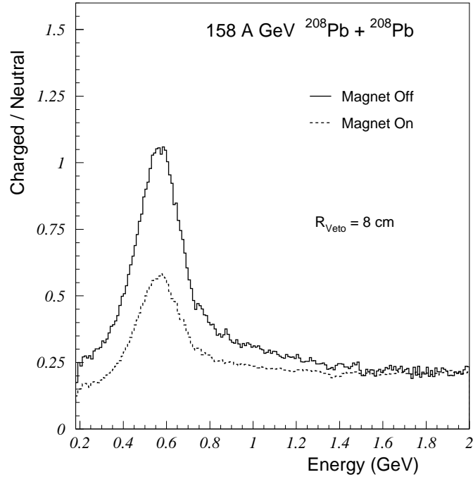
FIG. 8. The ratio of charged to neutral clusters identified in the lead-glass detector for peripheral collisions with magnet on or magnet off run conditions as a function of the total energy of the cluster in the low transverse momentum region. The solid curve shows the ratio for clusters identified as charged hits by a coincident hit in the CPV within a distance of R_{Veto} = 8 cm of the cluster. The peak at 550 MeV from non-showering minimum ionizing particles is clearly seen in the distributions. A minimum energy threshold of 750 MeV is used in the present analysis.
