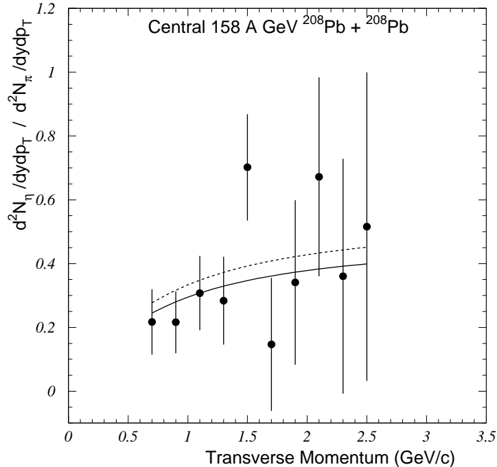
FIG. 25. The \eta/\pi^0 ratio as a function of transverse momentum for central 158 A GeV ^{208}\text{Pb}+^{208}\text{Pb} collisions. The solid curve is the ratio expected for m_T -scaling of the fitted \pi^0 result of Fig. 26 with a fitted normalization R_{\eta/\pi^0} = 0.486 . The dashed curve is the expected result with fixed normalization R_{\eta/\pi^0} = 0.55 .
