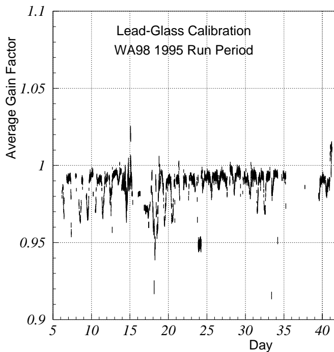
FIG. 3. The stability of the lead-glass calibration as determined with the LED monitoring system. The time-dependent gain factor, averaged over all modules, is shown as a function of time for the entire 1995 run period. The vertical size of the points indicates the rms of the distribution of time-dependent gains of all modules.
