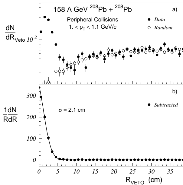
FIG. 6. The distribution of distances, R_{Veto} , to the nearest CPV hit from a shower particle in the lead-glass for peripheral events. In part a) the distribution for real events is shown by the solid circles. The distribution for randomly vetoed hits is shown by the open circles. The random veto distribution is obtained using test GEANT showers inserted into real events. The true veto radius distribution after subtraction of the random veto distribution is shown in part b).
