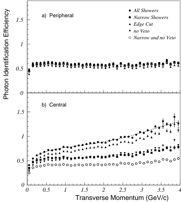
FIG. 14. The photon identification efficiency including effects of resolution, shower overlap, and excluded lead-glass modules as a function of transverse momentum for a) peripheral and b) central 158 A GeV ^{208}\text{Pb}+^{208}\text{Pb} collisions. The efficiencies are shown for several shower identification methods using the 1996 magnetic field on data. The efficiency is shown for the following criteria: all showers (solid circles), showers satisfying a dispersion cut (solid squares), all showers within a further restricted acceptance (solid triangles), all showers with no associated hit in the CPV (inverted solid triangles), and all showers satisfying a dispersion cut with no associated hit in the CPV (open circles). An example of the fitted parameterization of the efficiency is shown by the dashed curve in part b) for the criterion of using all showers.
