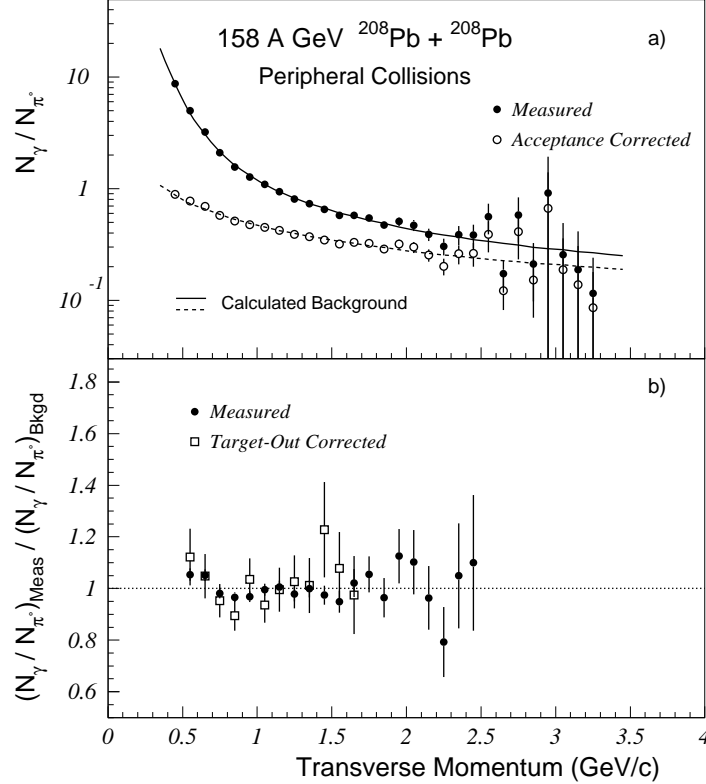
FIG. 29. The efficiency corrected (solid circles) and efficiency and acceptance corrected (open circles) \gamma/\pi^0 ratio is shown in part a) as a function of transverse momentum for peripheral 158 A GeV ^{208}\text{Pb}+^{208}\text{Pb} collisions. The calculated background (\gamma/\pi^0)_{\text{Bkgd}} ratio in the WA98 acceptance is shown by the solid curve. The dashed curve shows the calculated background with acceptance corrections. The ratio of measured (\gamma/\pi^0)_{\text{Meas}} ratio to calculated (\gamma/\pi^0)_{\text{Bkgd}} ratio for the WA98 acceptance is shown in part b). The errors on the data points indicate the statistical errors only.
