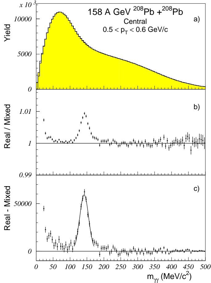
FIG. 18. The two-photon invariant mass distribution for central events in the \pi^0 mass region with pair transverse momentum 0.5 < p_T < 0.6 \text{ GeV}/c . Results are shown for the 1995 magnet on data sample. Part a) shows the invariant mass distribution for all shower pairs for real events (solid histogram) and mixed events (filled histogram). Part b) shows the ratio of real and mixed event mass distributions. Part c) shows the real invariant mass distribution after subtracting the normalized mixed event distribution.
