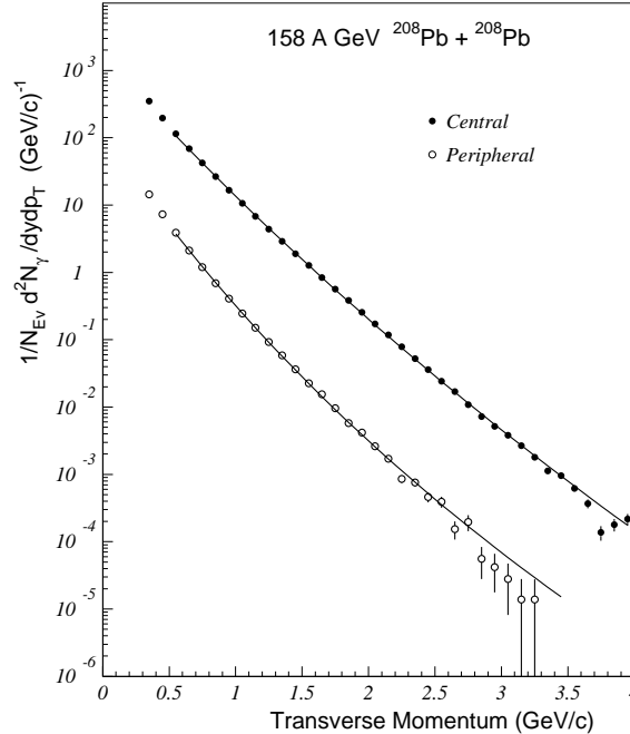
FIG. 27. The inclusive photon transverse momentum distribution for peripheral (open circles) and central (solid circles) 158 A GeV ^{208}\text{Pb}+^{208}\text{Pb} collisions for the sum of 1995 and 1996 magnet on data sets. The narrow shower photon identification criterion has been used. The data have been corrected for efficiency and acceptance. Only statistical errors are shown. The solid curves show the fit results described in the text.
