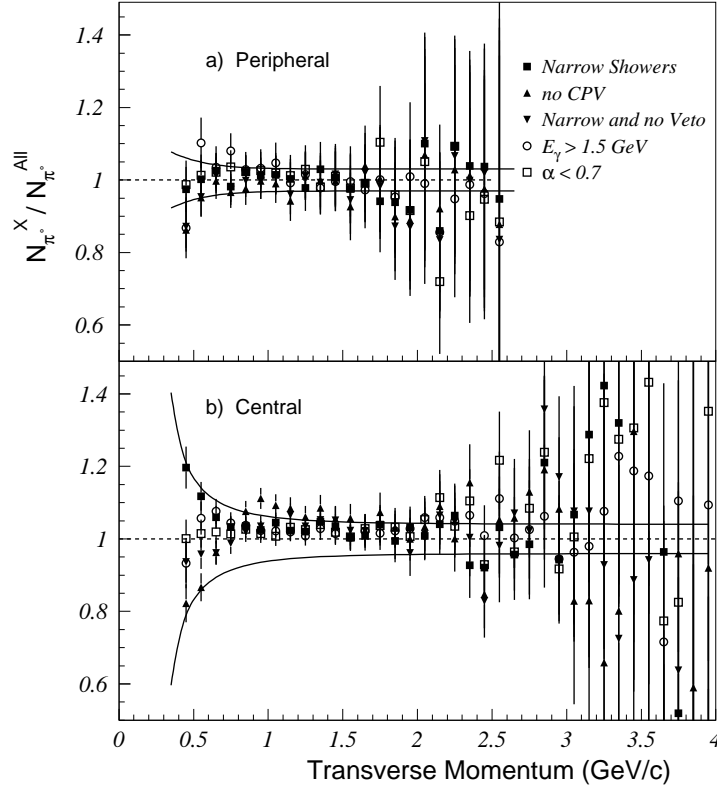
FIG. 23. The ratio of the efficiency-corrected \pi^0 yield for various shower identification methods compared to the method of using all showers is shown as a function of transverse momentum. The results are shown for a) peripheral and b) central 158 A GeV ^{208}\text{Pb}+^{208}\text{Pb} collisions for the 1996 data set. The error bars indicate statistical errors only. The horizontal lines indicate the estimated systematical errors. The deviation from unity, beyond statistical error, is indicative of the systematical error in the \pi^0 yield extraction.
