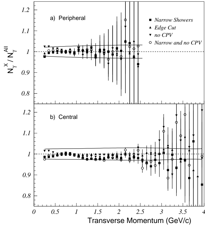
FIG. 15. The ratio of the efficiency-corrected inclusive photon yield for various methods compared to the method of using all showers ( N_\gamma^{All} ) is shown as a function of transverse momentum. The results are shown for a) peripheral and b) central 158 A GeV ^{208}\text{Pb}+^{208}\text{Pb} collisions for the 1996 magnet on data set. The error bars indicate statistical errors only. The deviation from unity, beyond statistical error, is indicative of the systematical error attributed to the photon identification method. The horizontal lines indicate the estimated systematical error on the photon yield determination.
