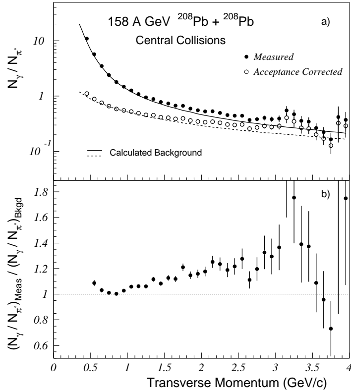
FIG. 30. The efficiency corrected (solid circles) and efficiency and acceptance corrected (open circles) \gamma/\pi^0 ratio is shown in part a) as a function of transverse momentum for central 158 A GeV ^{208}\text{Pb} + ^{208}\text{Pb} collisions. The calculated background (\gamma/\pi^0)_{\text{Bkgd}} ratio in the WA98 acceptance is shown by the solid curve. The dashed curve shows the calculated background with acceptance corrections. The ratio of measured (\gamma/\pi^0)_{\text{Meas}} ratio to calculated (\gamma/\pi^0)_{\text{Bkgd}} ratio for the WA98 acceptance is shown in part b). The errors on the data points indicate the statistical errors only.
