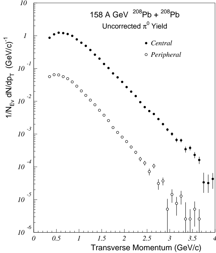
FIG. 20. The uncorrected \pi^0 multiplicity as a function of the transverse momentum for peripheral (open circles) and central (solid circles) 158 A GeV ^{208}\text{Pb}+^{208}\text{Pb} collisions. The results are for the full magnet on data sample. Narrow showers with energy above 750 MeV have been used in the invariant mass calculation. The data have not been corrected for efficiency or acceptance. These spectra are used as the first iteration in the iterative efficiency correction.
