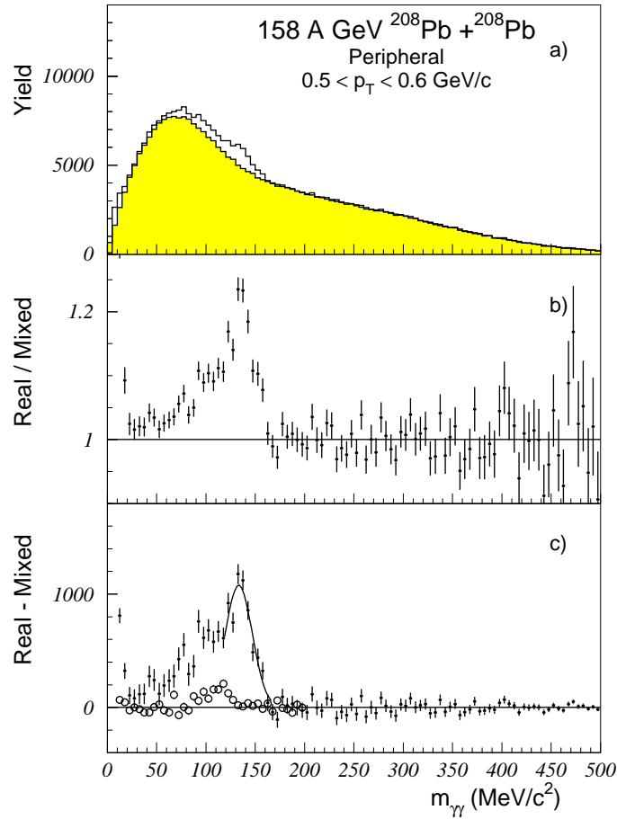
FIG. 16. The two-photon invariant mass distribution for peripheral events in the \pi^0 mass region with pair transverse momentum 0.5 < p_T < 0.6 GeV/c. Results are shown for the 1996 magnet on data sample. Part a) shows the invariant mass distribution for all shower pairs for real events (solid histogram) and mixed events (filled histogram). Part b) shows the ratio of real and mixed event mass distributions. Part c) shows the real invariant mass distribution after subtracting the normalized mixed event distribution. The normalized target out background contribution is shown by the open circles in part c).
