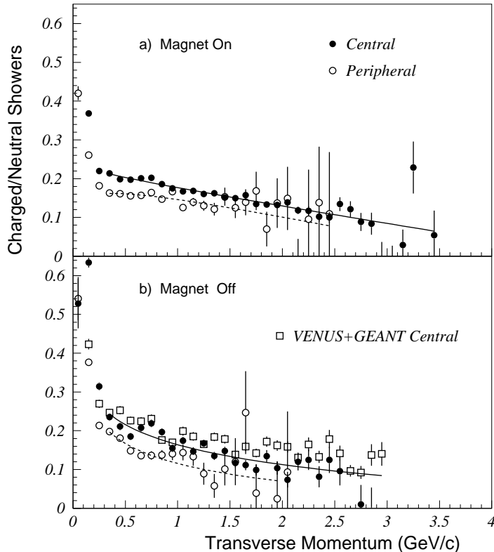
FIG. 10. The measured ratio of charged to neutral showers in the lead-glass detector for peripheral (open circles) and central (solid circles) 158 A GeV ^{208}\text{Pb}+^{208}\text{Pb} collisions as a function of the transverse momentum of the cluster. The results are shown for all clusters for a) magnet on and b) magnet off. The data have been corrected for photon conversions and the CPV efficiency. The lines are fitted curves.
