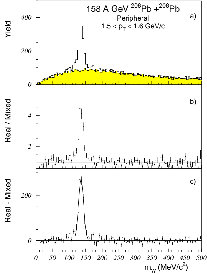
FIG. 17. The two-photon invariant mass distribution for peripheral events in the \pi^0 mass region with pair transverse momentum 1.5 < p_T < 1.6 GeV/c. Results are shown for the 1995 magnet on data sample. Part a) shows the invariant mass distribution for all shower pairs for real events (solid histogram) and mixed events (filled histogram). Part b) shows the ratio of real and mixed event mass distributions. Part c) shows the real invariant mass distribution after subtracting the normalized mixed event distribution.
