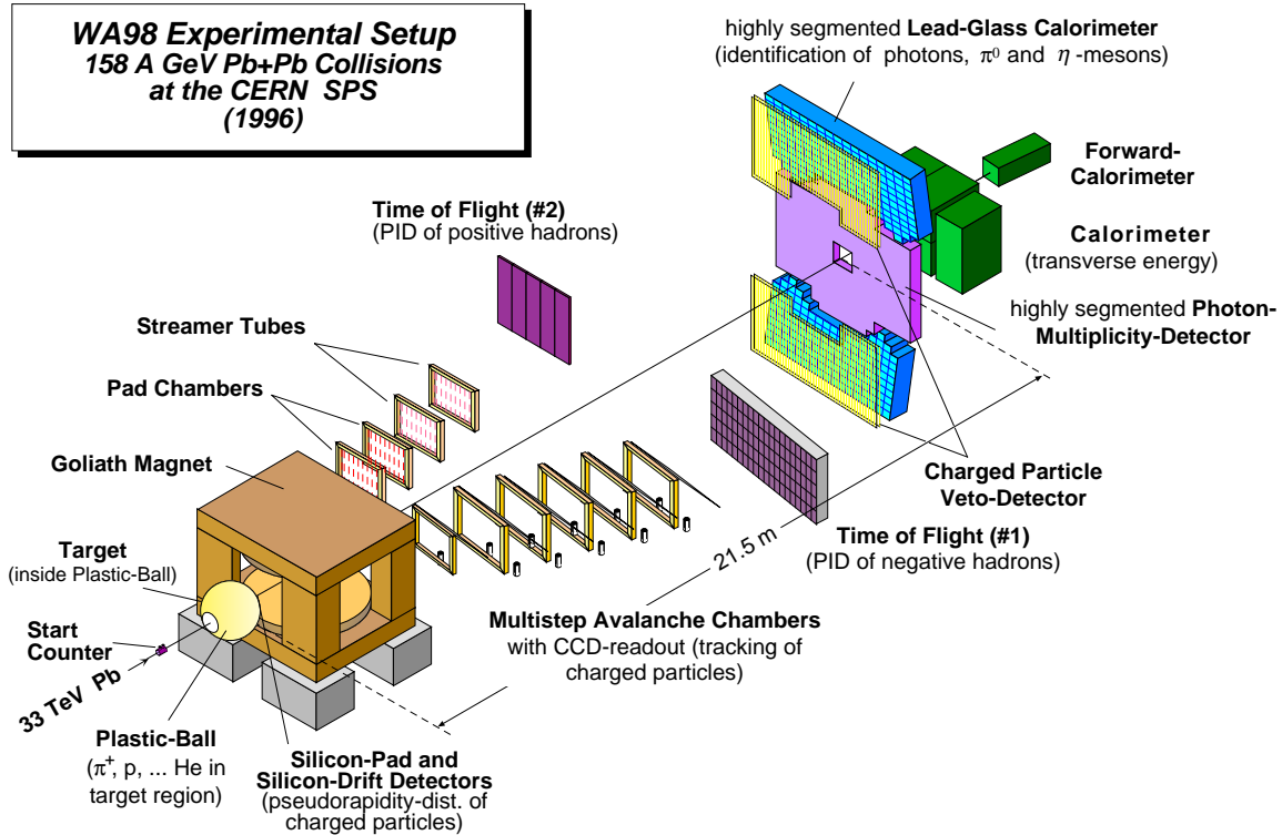
FIG. 1. The WA98 experimental setup.
