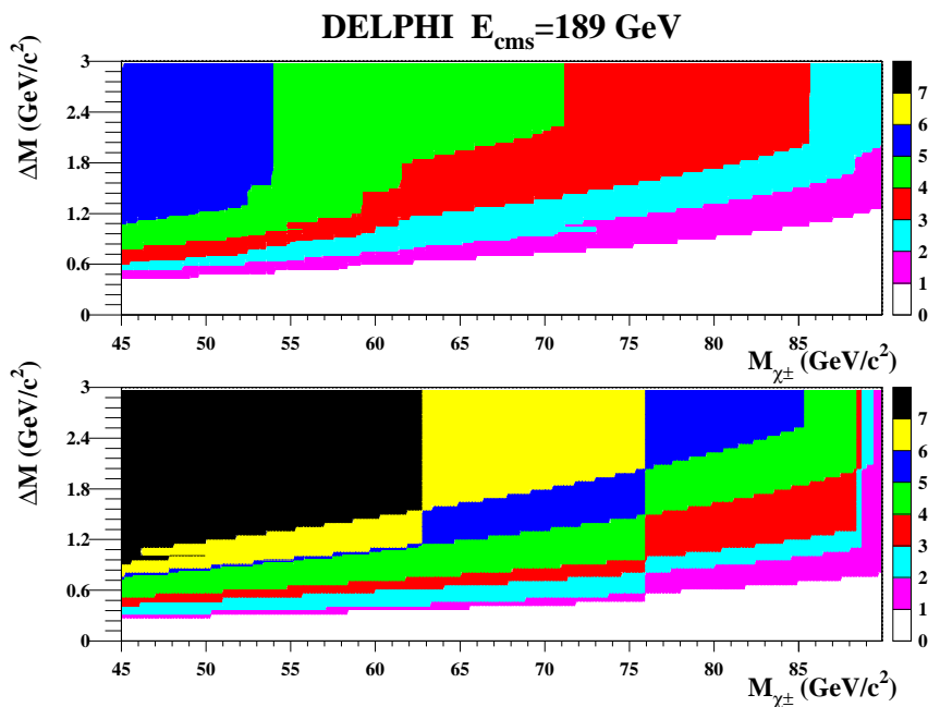
Figure 4: SM MC (top) and data (bottom) remaining after the final selection in any point of the plane (M_{\tilde{\chi}_1^\pm}, \Delta M) considered in the search with the ISR photon at 189 GeV.
