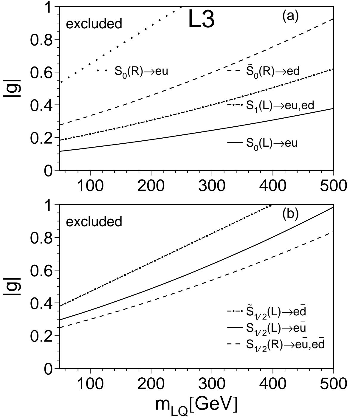
Figure 3: The 95% confidence level upper limits on |g_L| or |g_R| as a function of m_{LQ} for various scalar leptokuarks derived from hadronic final state cross sections. Limits are shown for fermion number F=2 (a) and for F=0 (b). Bounds on the R-parity violating couplings |\lambda'_{1jk}| for the exchange of scalar down-type quarks in the u -channel and scalar up-type quarks in the t -channel correspond to limits on |g_L| for the S_0(L) and \tilde{S}_{1/2} leptokuark exchange, respectively.
