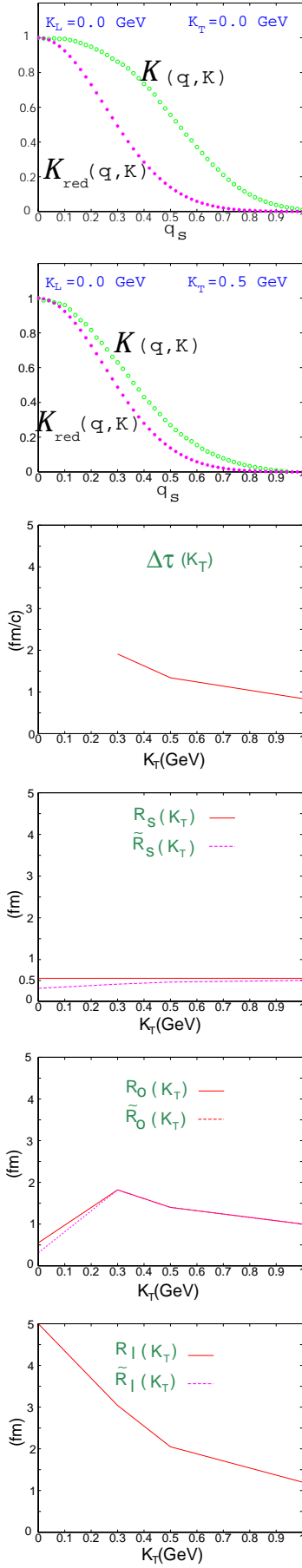
Figure 1: First two panels: The correlation function in side-direction ( q_o = q_l = 0 ) for pairs with K_L = 0 (such that the R_{ol} cross term vanishes 1 ) and K_T = 0 and 0.5 GeV, respectively. Third panel: The emission time duration \Delta\tau = \sqrt{R_o^2 - R_s^2}/\beta_T as a function of K_T for K_L = 0 . Second row: R_s , R_o , and R_l as functions of K_T for K_L = 0 . We checked that the HBT radii correctly reproduce the rms widths of the space-time scatter plots of the produced pions in the appropriate \mathbf{K} -windows.
