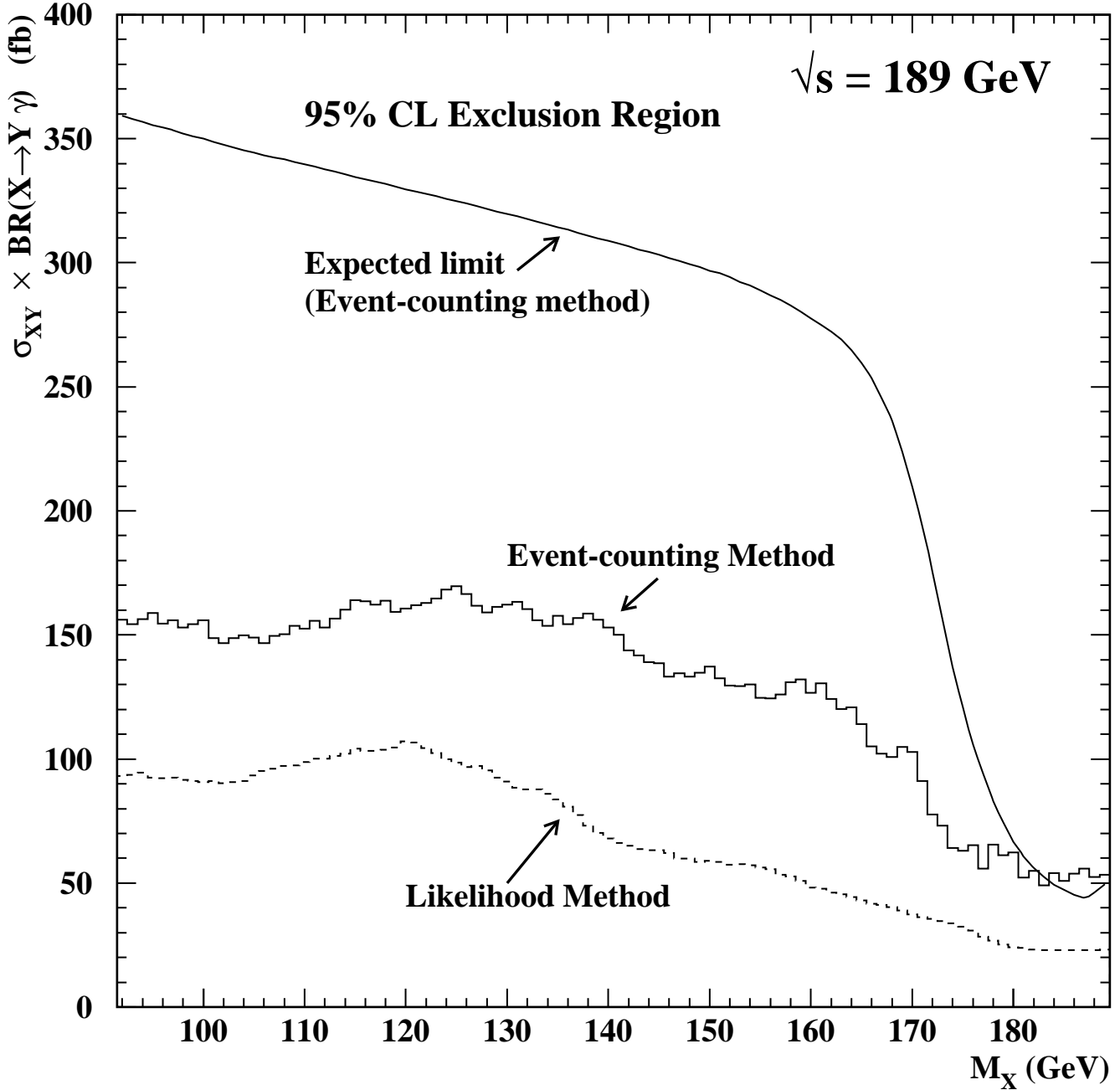
Figure 11: The 95% CL upper limits on \sigma(e^+e^- \rightarrow XY) \cdot \text{BR}(X \rightarrow Y\gamma) at \sqrt{s} = 189 \text{ GeV} as a function of M_X , assuming M_Y \approx 0 , calculated using the likelihood-based method and the event-counting method as described in the text. Also shown is the average limit expected in the absence of signal, calculated using the event-counting method.
