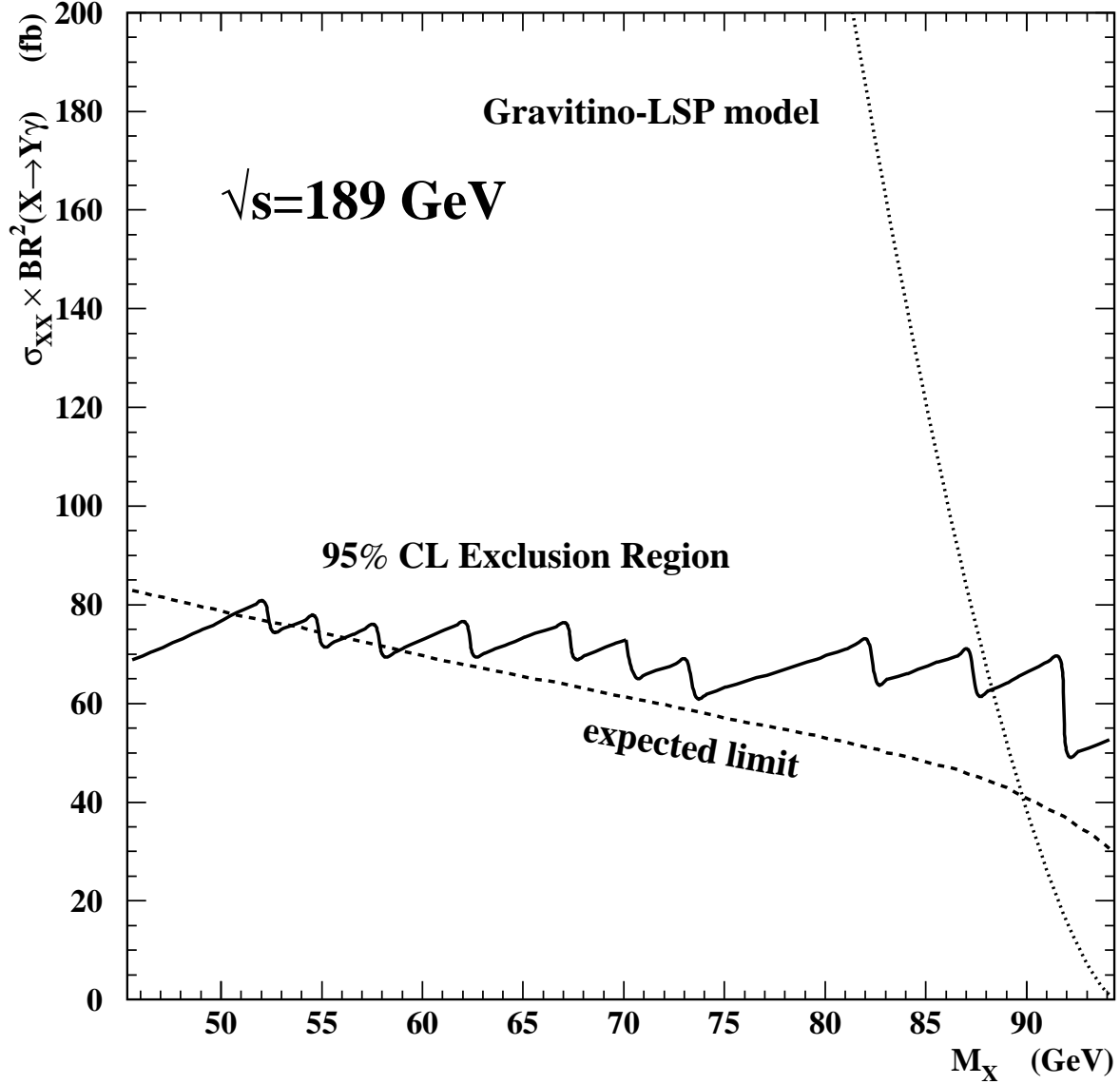
Figure 14: 95% CL upper limit on \sigma(e^+e^- \rightarrow XX) \cdot \text{BR}^2(X \rightarrow Y\gamma) for M_Y \approx 0 (solid line). Also shown is the expected limit (dashed line). The dotted line shows the cross-section prediction of a specific light gravitino LSP model [30]. Within that model, \tilde{\chi}_1^0 masses between 45 and 88.3 GeV are excluded at the 95% CL. These limits assume that particle X decays promptly.
