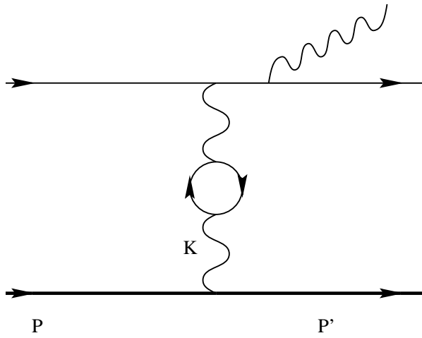
FIG. 2. Example for a scattering diagram related to the imaginary part of the diagram in Fig.1
