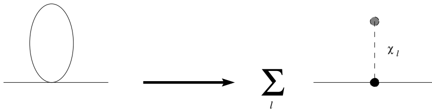
Figure 2: Dual-channel interpretation of the thermal loop in the planar contribution to the two-point function in \phi^4 non-commutative field theory.
