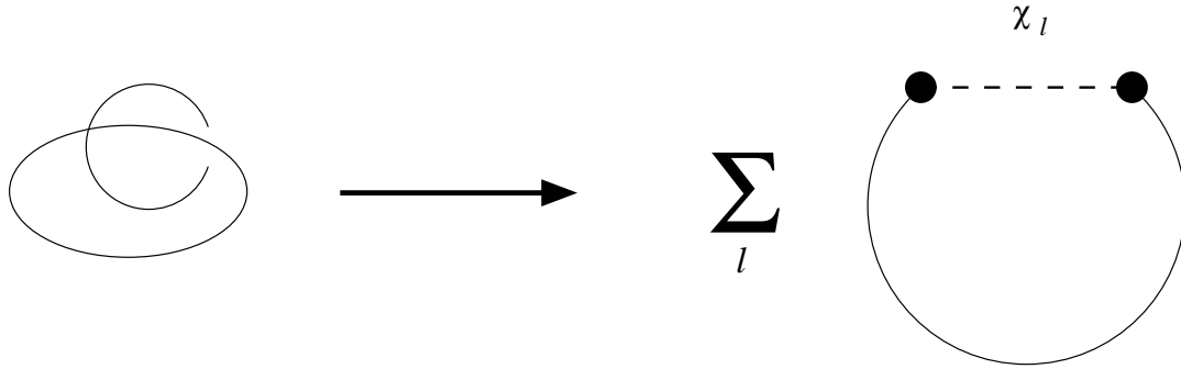
Figure 4: Dual-channel description of the non-planar thermal loop in \phi^4 -like two-loop non-planar vacuum diagram.
