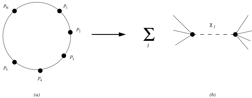
Figure 3: Channel duality for a non-planar thermal loop in \phi^n non-commutative field theory.
