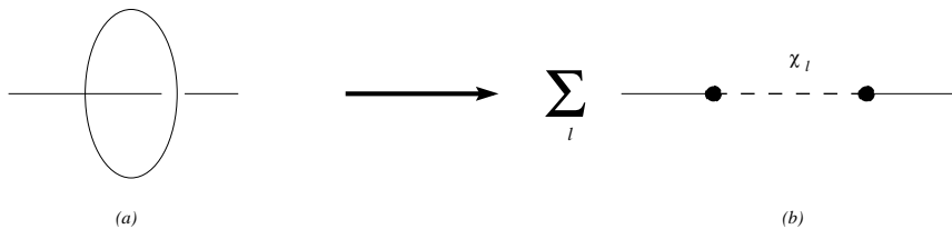
Figure 1: “Channel duality” in the non-planar self-energy diagram in \phi^4 theory.
