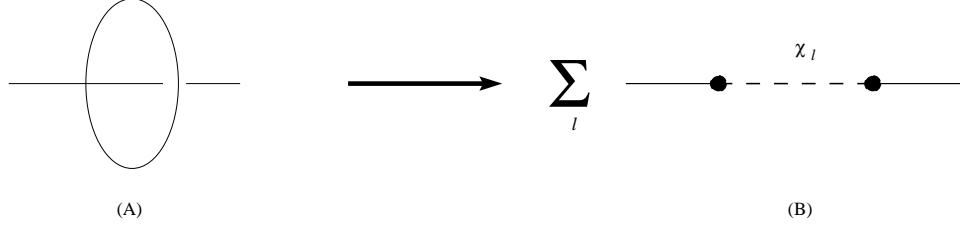
Fig. 1: ‘Channel duality’ in the nonplanar self-energy diagram in d = 4 theory.
