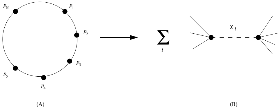
Fig. 3: Channel duality for a nonplanar thermal loop in \mathcal{N}=n noncommutative field theory.
