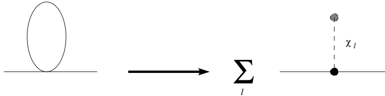
Fig. 2: Dual channel interpretation of the thermal loop in the planar contribution to the two-point function in \alpha'^4 noncommutative eld theory.
