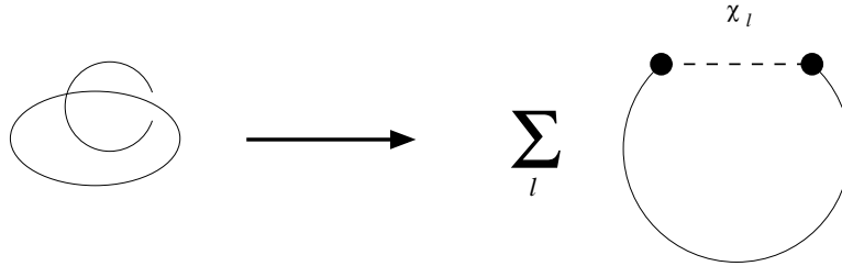
Fig. 4: Dual channel description of the nonplanar thermal loop in d = 3 -like two-loop nonplanar vacuum diagram.
