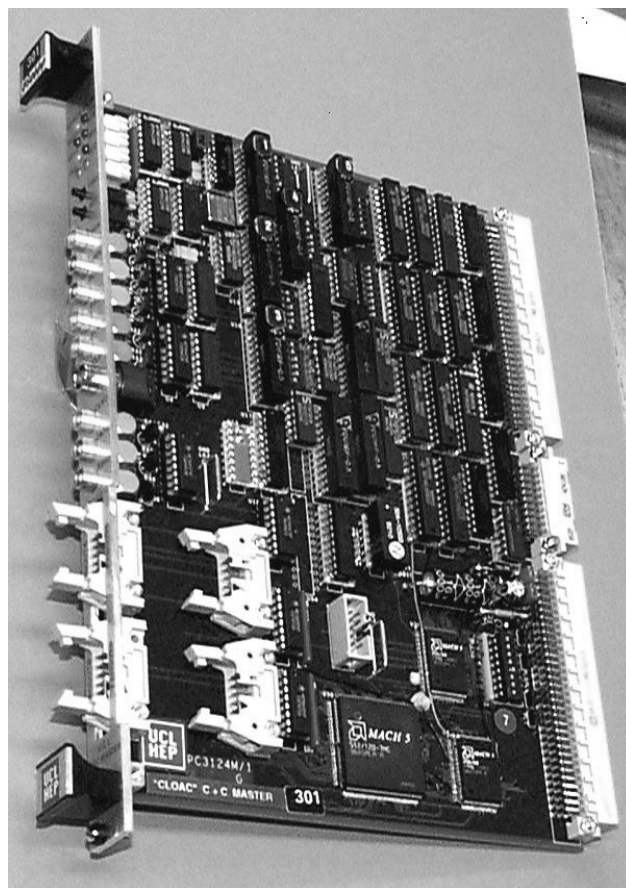
Fig. 5 : Picture of CLOAC MASTER module
