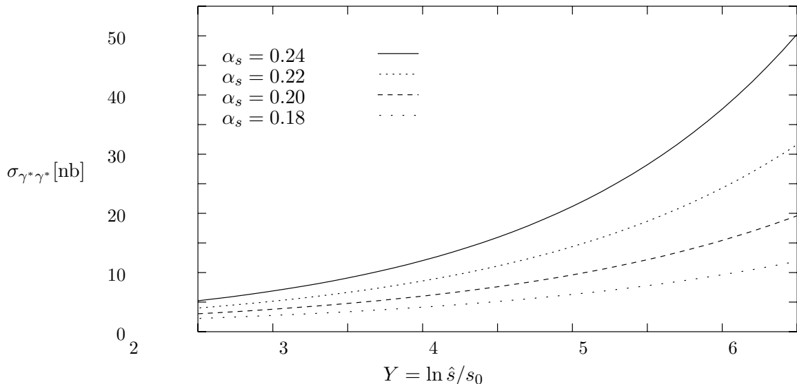
Figure 4: Same as Fig. 3, here for LEP183 with \langle Q^2 \rangle = 14 \text{ GeV}^2
