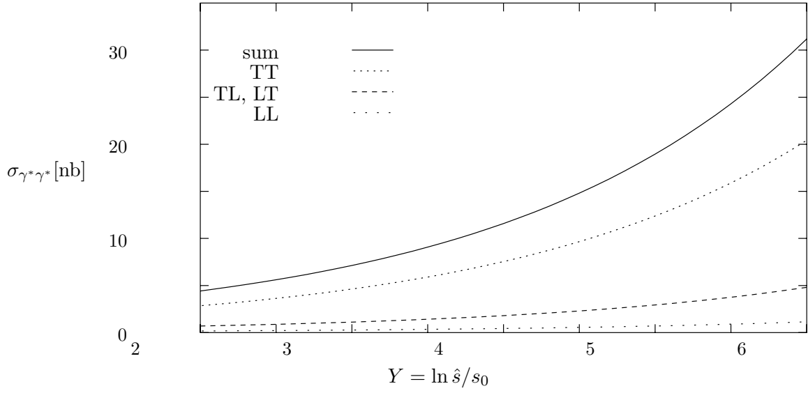
Figure 2: Contributions of different photon polarizations to the cross section, here for LEP 183 with \langle Q^2 \rangle = 14 \text{ GeV}^2 , \alpha_s = 0.208 , m_c = 0
