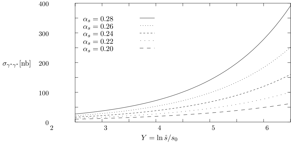
Figure 3: Energy dependence of the \gamma^*\gamma^* cross section for different values of \alpha_s(\langle Q^2 \rangle) , here for LEP91 with \langle Q^2 \rangle = 3.5 \text{ GeV}^2 , m_c = 1.5 \text{ GeV} .
