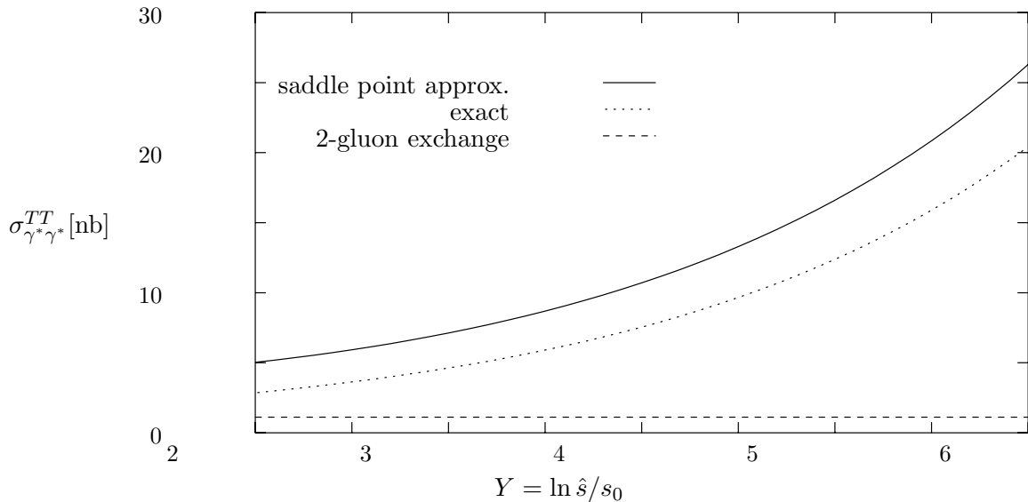
Figure 1: Comparison of the exact BFKL result with the saddle point approximation and the two–gluon exchange approximation for transversely polarized photons at LEP183 with \langle Q^2 \rangle = 14 \text{ GeV}^2 , \alpha_s = 0.208
