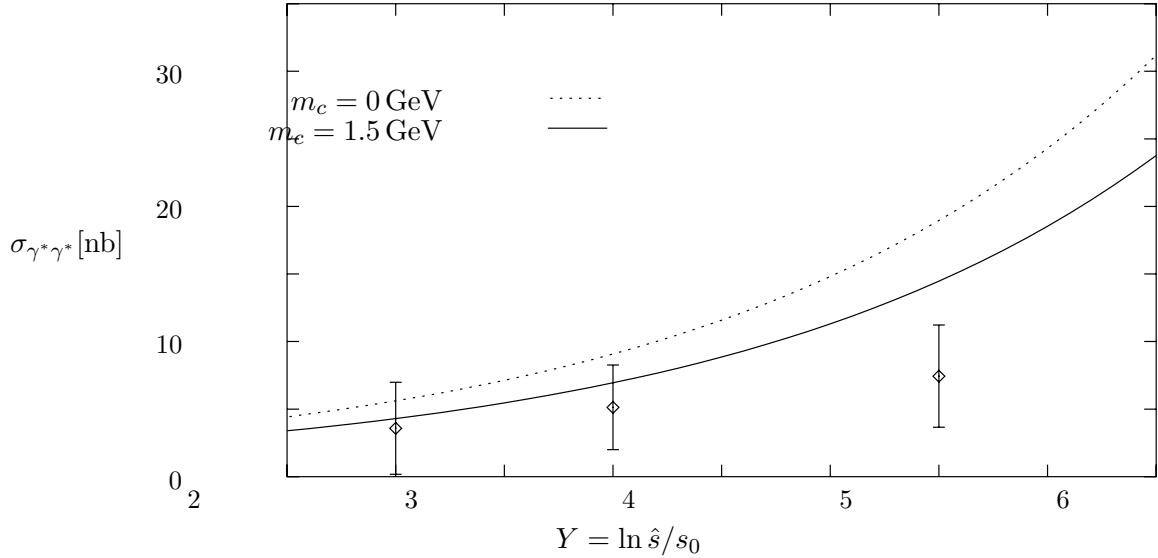
Figure 6: Same as Fig. 5, here for LEP183 with \langle Q^2 \rangle = 14 \text{ GeV}^2 , \alpha_s = 0.208
