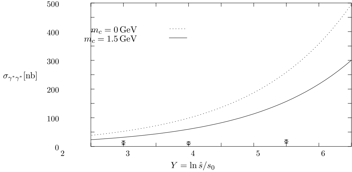
Figure 5: Effect of the charm quark mass on the \gamma^*\gamma^* cross section for LEP 91 with \langle Q_i^2 \rangle = 3.5 \text{ GeV}^2 , \alpha_s = 0.268 . Data points as measured by the L3 collaboration [2].
