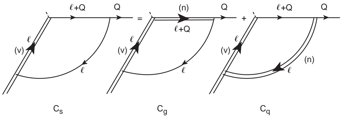
Figure 5: Second decomposition in T_{\mu\nu} . The thin and double lines represent the massless quadratic and eikonal propagators, respectively. The symbols (v) and (n) indicate that the eikonal propagators must be taken along the directions v and n .
