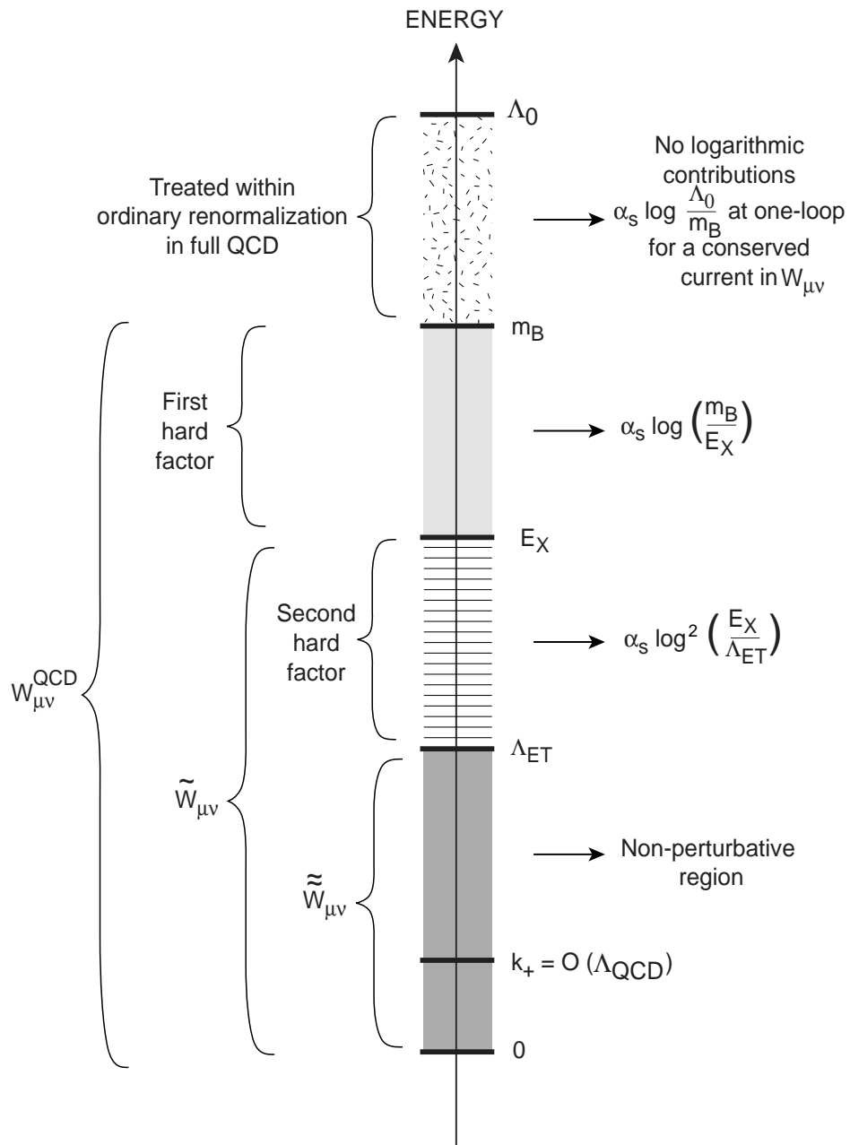
Figure 1: Pictorial description of factorization in the effective theory.
