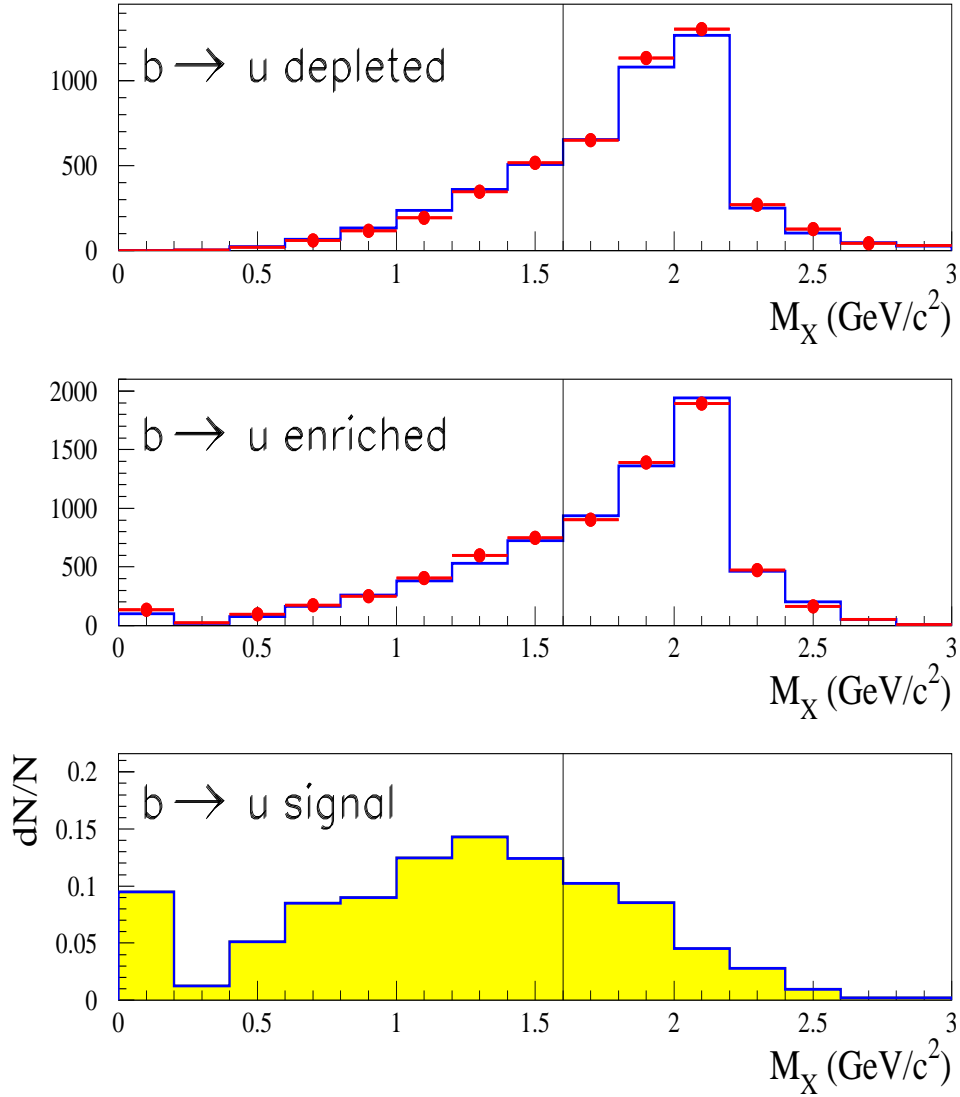
Figure 5: Invariant mass M_X of the reconstructed secondary hadronic system in selected decays for data (points with error bars) and simulation (histogram). The plots show the b \rightarrow u depleted sample (upper plot), the b \rightarrow u enriched sample (medium plot) and the b \rightarrow u signal (lower plot). The vertical lines correspond to the value chosen for the low M_X selection.
