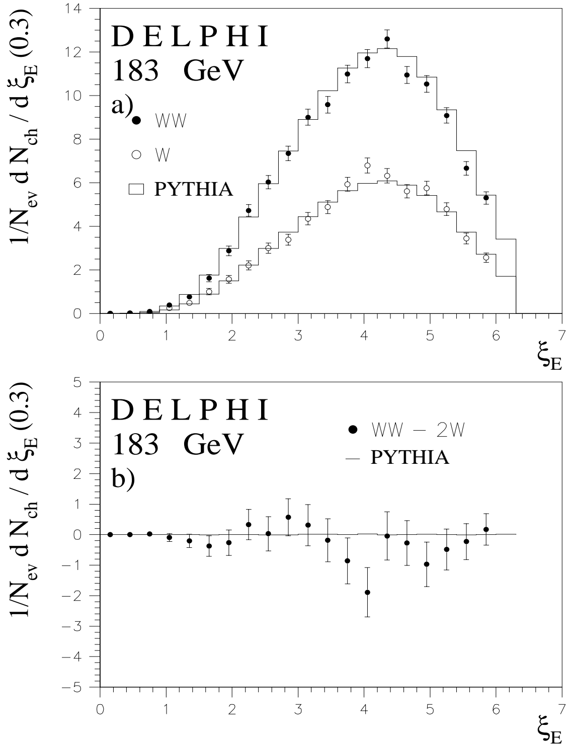
Figure 5: (a) Corrected \xi_E distributions of charged particles for (4q) events (closed circles) and (2q) events (open circles), at 183 GeV, compared to simulation without colour reconnection. The error bars in the data represent the statistical errors. The difference between (4q) and twice (2q) is shown in (b).
