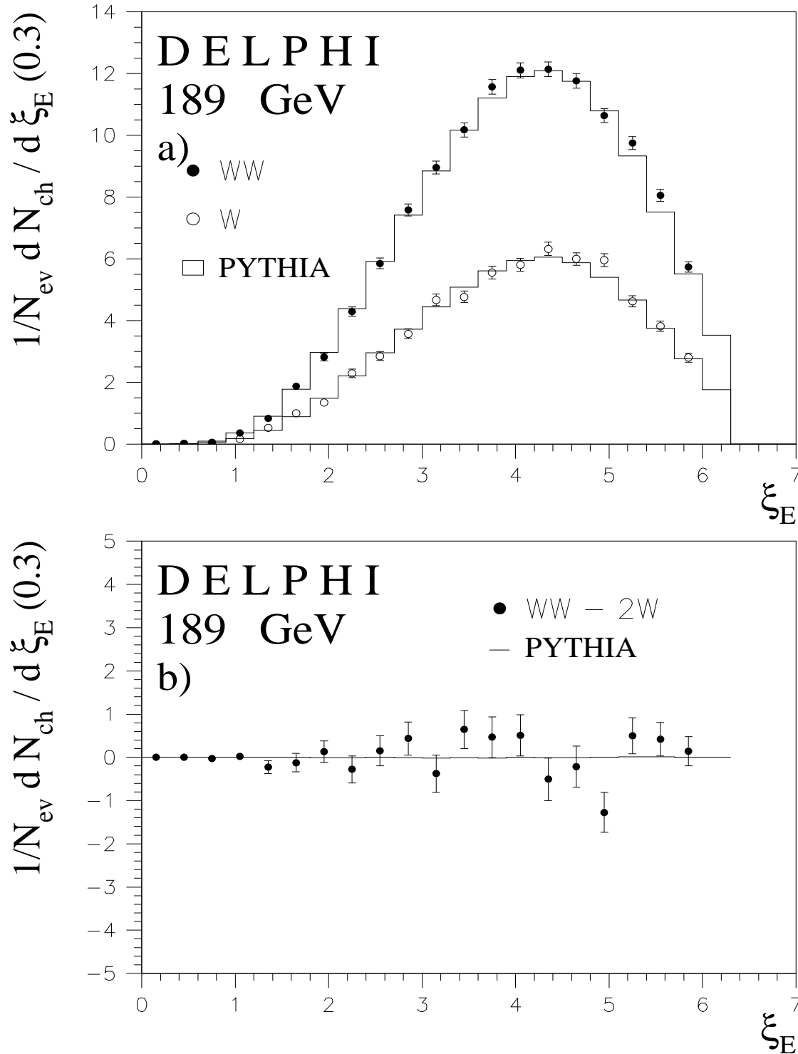
Figure 4: (a) Corrected \xi_E distributions of charged particles for (4q) events (closed circles) and (2q) events (open circles), at 189 GeV, compared to simulation without colour reconnection. The error bars in the data represent the statistical errors. The difference between (4q) and twice (2q) is shown in (b).
