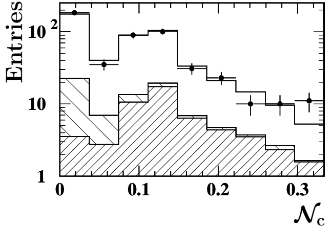
Figure 6: The \mathcal{N}_b , \mathcal{N}_c , and \mathcal{N}_{bc} distributions for lepton and slow pion tagged events at 189 GeV centre-of-mass energy. The points with error bars correspond to the data. The open histogram represents the Monte Carlo expectation, where the contributions from signal events are shown hatched as explained in the figure. The purity in the slow pion selection is limited, which is reflected in the fact that the range of \mathcal{N}_c and \mathcal{N}_{bc} values for slow pions does not extend up to 1.
