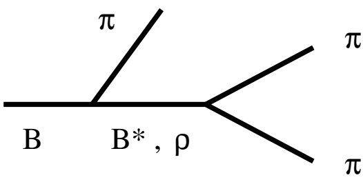
Fig. 1 - The polar diagram. For the B resonances ( B^* = 1^-, 0^+ ) the strong coupling is on the left and the weak coupling on the right; the situation is reversed for the \rho production.
