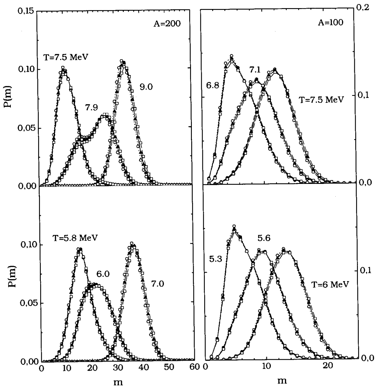
FIG. 11. The total fragment multiplicity distributions. For further details see the caption of Fig. 10.
