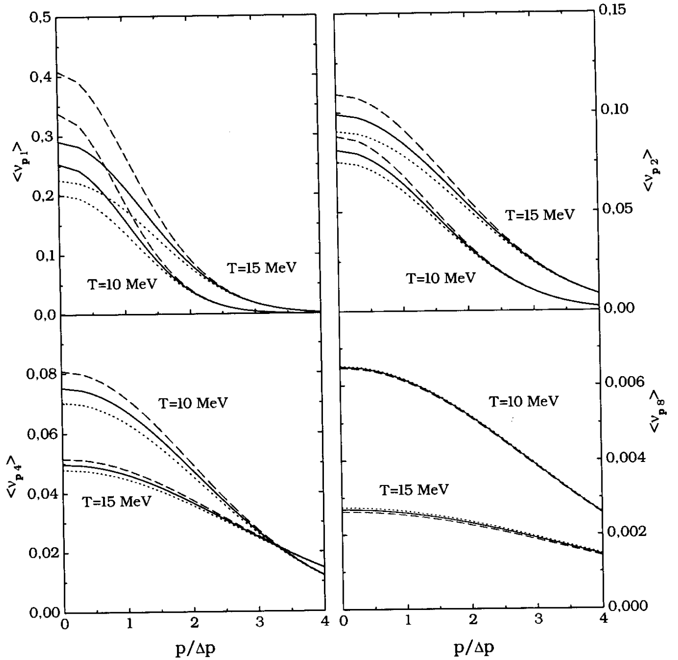
FIG. 1. The mean occupation numbers \langle \nu_{\vec{p}_i} \rangle of fragments of mass i for A = 200 system at temperatures of 10 and 15 MeV. The dashed, dotted and continuous curves correspond to the QSM result obtained under the assumption that all fragments are bosons, fermions or Boltzmann particles, respectively. The system volume is V/V_0 = 3 and \Delta p = 90 MeV/c.
