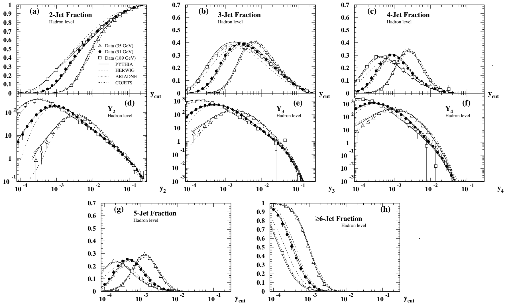
Figure 2: In plots (a), (b), (c), (g) and (h), the fractions of events with 2, 3, 4, 5 and more than 5 jets as obtained by the Durham scheme are plotted versus y_{cut} at 35, 91 and 189 GeV. Diagrams (d) through (f) show the distributions in y_n (see Sect. 4.2.2) corresponding to (a), (b) and (c). The presentation is the same as in Fig. 1. Small horizontal ticks indicate the size of the statistical errors.
