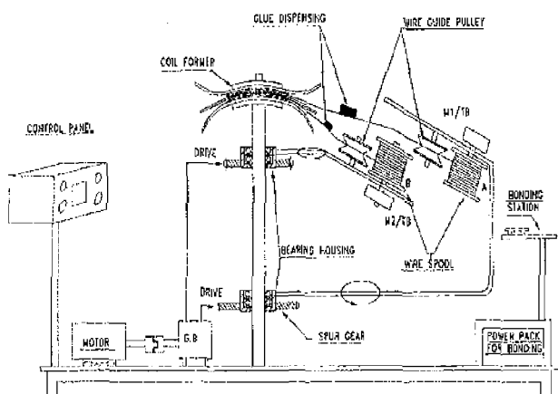
Fig. 1. Tilted-arm automatic coil winding machine.
