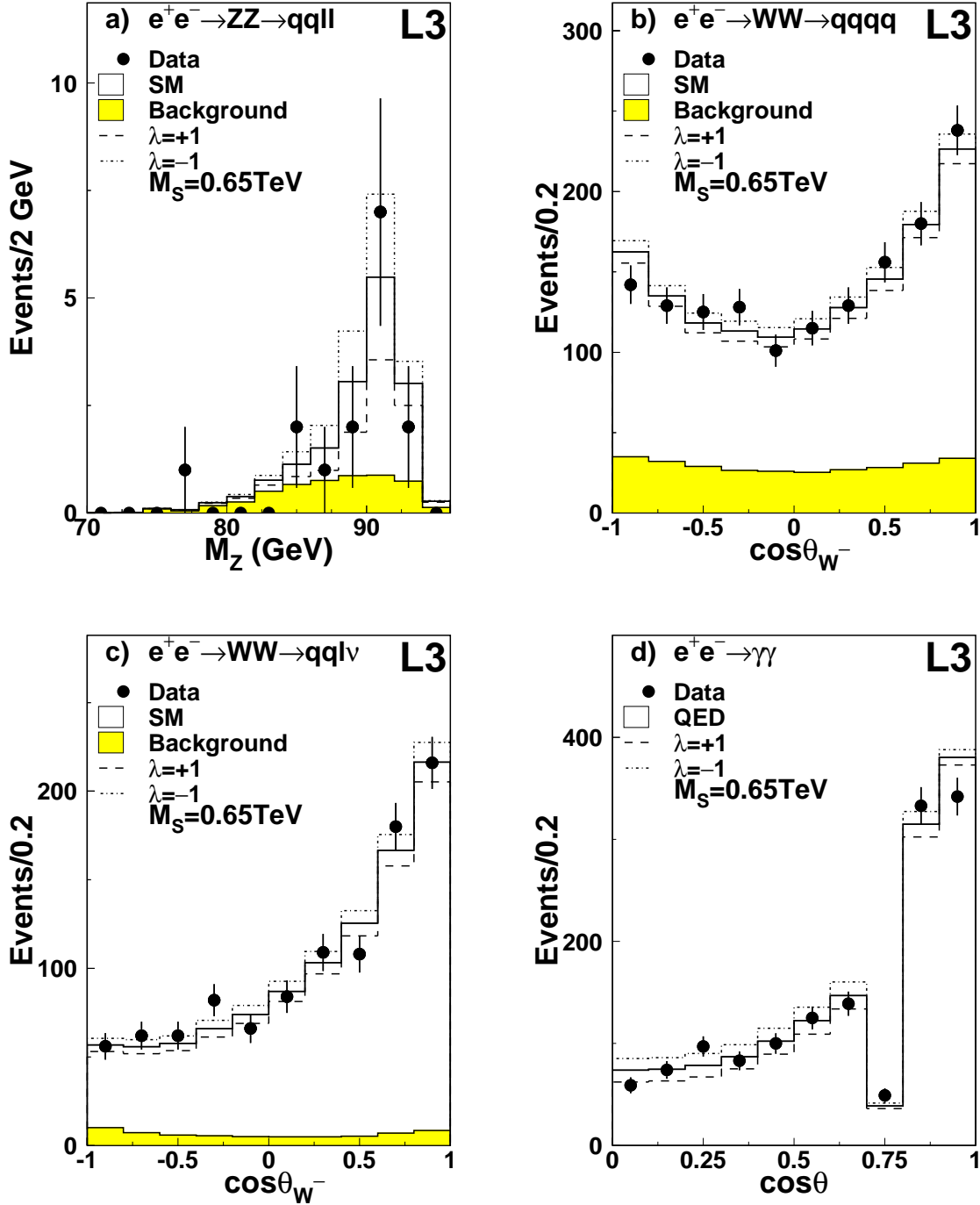
Figure 1: (a) Reconstructed Z mass for e^+e^- \rightarrow ZZ \rightarrow qq\bar{\ell}^+\ell^- events. Distributions of the polar angle for: (b) hadronic e^+e^- \rightarrow W^+W^- events, (c) semileptonic e^+e^- \rightarrow W^+W^- events, (d) e^+e^- \rightarrow \gamma\gamma events. Data at 188.7 GeV, SM signal and background expectations are presented together with LSG predictions for M_S = 0.65 \text{ TeV} and \lambda = \pm 1 .
