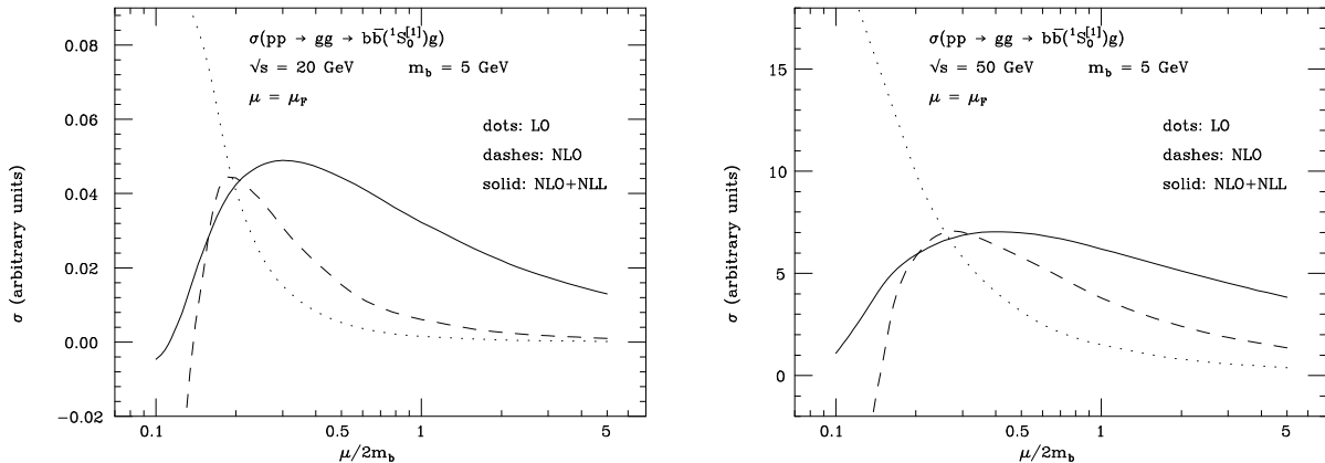
Figure 4: The cross sections for production of the bottomonium state ^1S_0^{[1]} via the gluon–gluon channel, at 20 and 50 GeV centre-of-mass energy, as functions of the renormalization/factorization scales.
