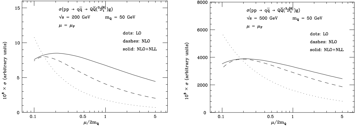
Figure 2: The cross section for production, in pp collisions via the q\bar{q} channel, of a {}^3S_1^{[8]} state with 50 GeV quarks.
