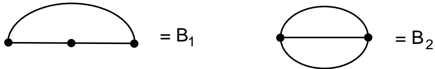
Fig. 2: Diagrams that contribute to I_{an}^{(m,n)} with m+n=3 .
