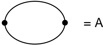
Fig. 1: The diagram that contributes to I_{an}^{(m,n)} with m + n = 2 .
