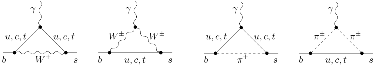
Figure 4: One-loop 1PI diagrams for b \rightarrow s\gamma in the SM. The charged would-be Goldstone boson is denoted by \pi^\pm . There is no W^\pm\pi^\mp\gamma coupling in the background-field gauge.
