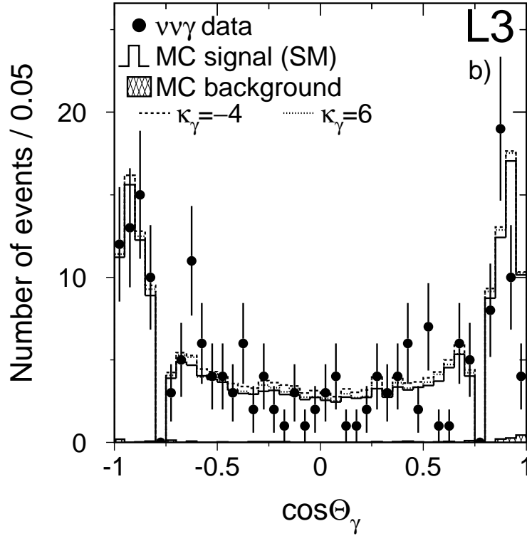
Figure 4: Distributions of a) the energy, E_\gamma , and b) the polar angle, \Theta_\gamma , of the photon in single-photon events. The data collected at \sqrt{s} = 183 GeV are shown, together with the expectations for the SM ( \kappa_\gamma = 1 ), and for anomalous TGCs ( \kappa_\gamma = -4 or 6 ). The main sensitivity of single-photon events to TGCs occurs at large photon energies.
