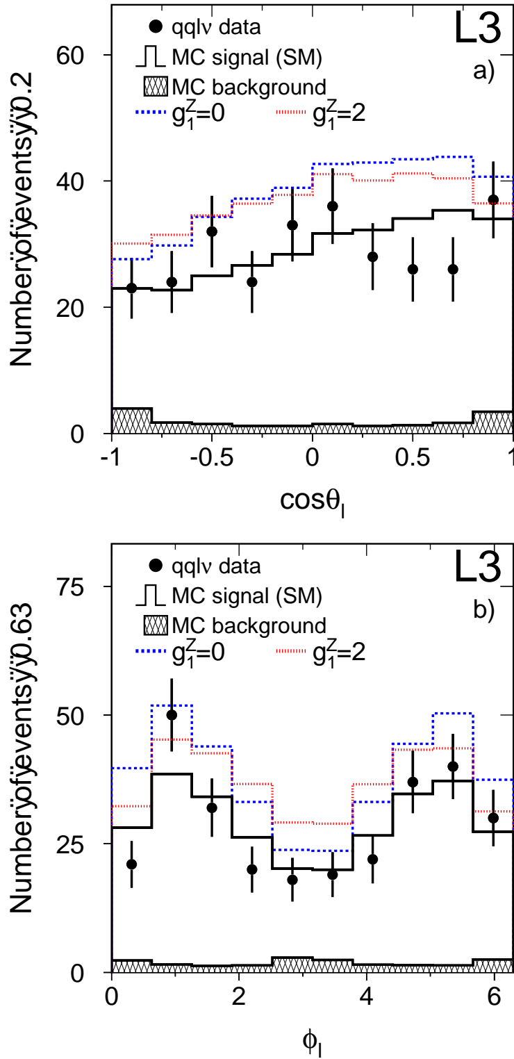
Figure 2: Distributions of the reconstructed W decay angles in qq\bar{l}\nu W-pair events, a) \cos\theta_\ell and b) \phi_\ell . The data collected at \sqrt{s} = 183 GeV are shown, together with the expectations for the SM ( g_1^Z = 1 ), and for anomalous TGCs, ( g_1^Z = 0 or 2 ). The \phi_\ell distribution for W^- decays is shifted by \pi in order to have the same \phi_\ell distribution for W^- and W^+ decays.
