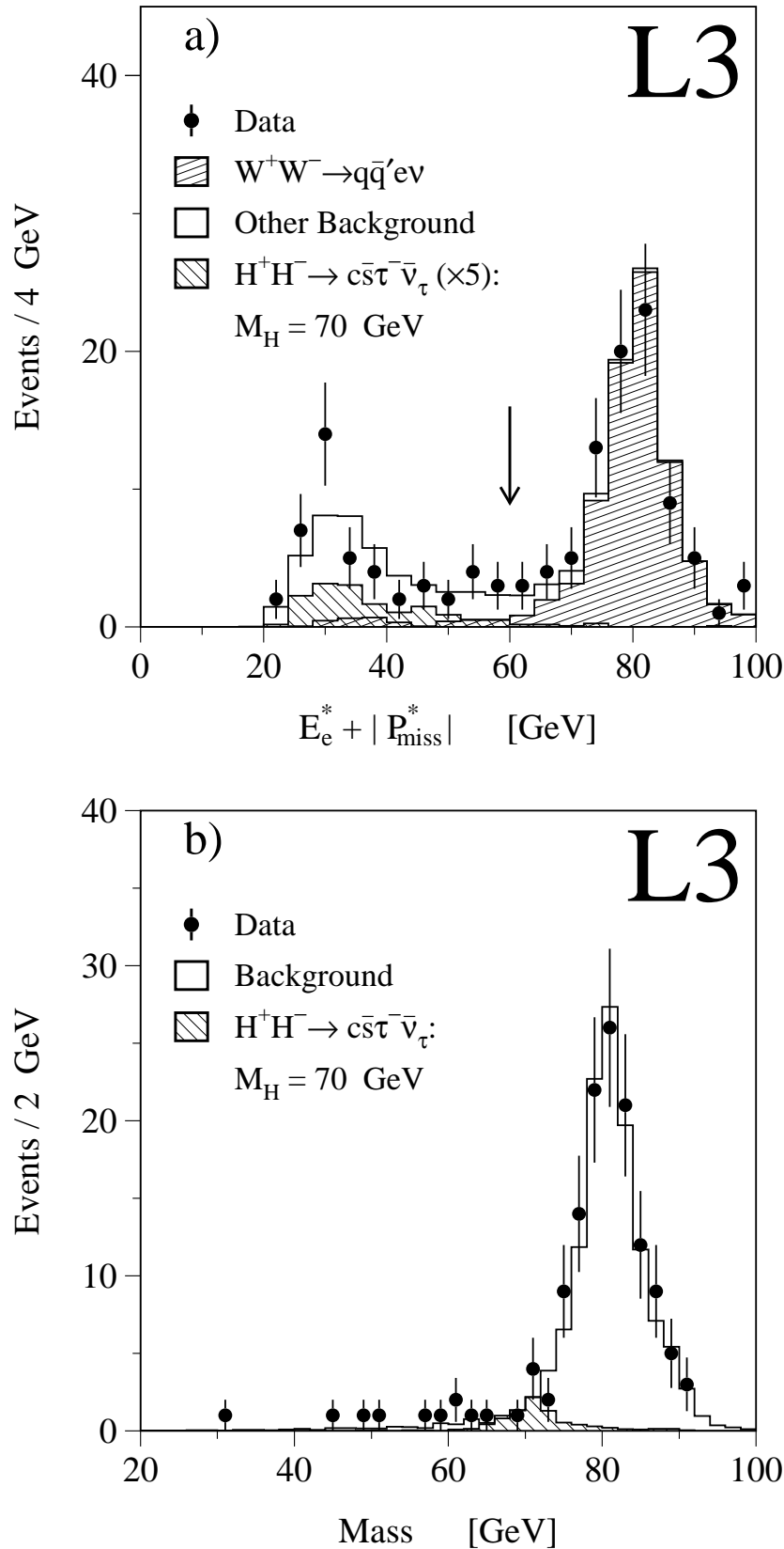
Figure 2: Distributions for the H^+H^- \rightarrow c\bar{s}\tau^-\bar{\nu}_\tau channel. a) E_e^* + |P_{\text{miss}}^*| for events with an identified electron in the final state after all other cuts, the arrow indicates the position of the cut. b) Reconstructed mass spectrum after all cuts. The expected distribution for a 70 GeV Higgs at \text{Br}(H^\pm \rightarrow \tau\nu) = 0.5 is superimposed, multiplied by a factor five in a).
