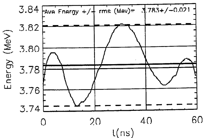
Fig. 3 Injector energy spread with expanded scale
