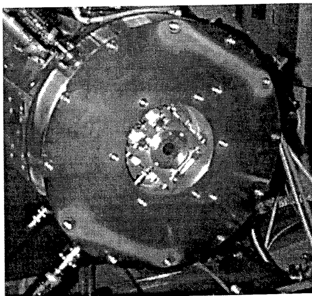
Figure 1: RFQ endflange with permanent magnet quadrupole.
