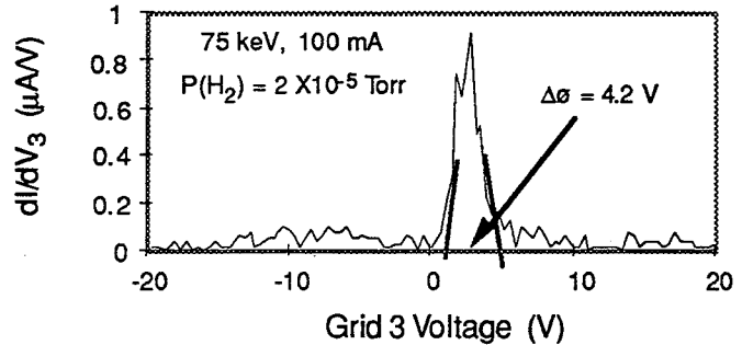
Fig. 3. Measurement of the energy distribution of positively charged particles expelled from the beam plasma.
