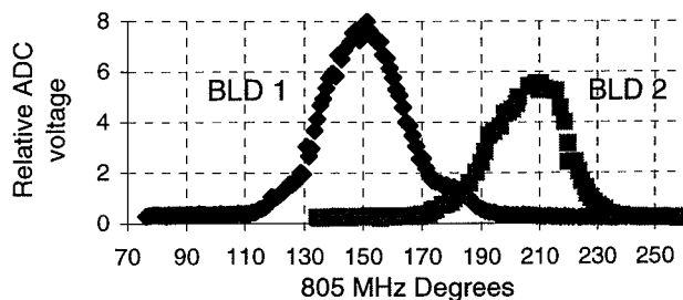
Figure 3, Typical bunch-length measurement.
