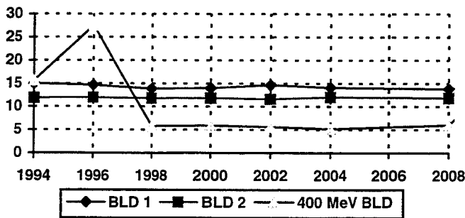
Figure 4, Bunch Length through the macropulse.
