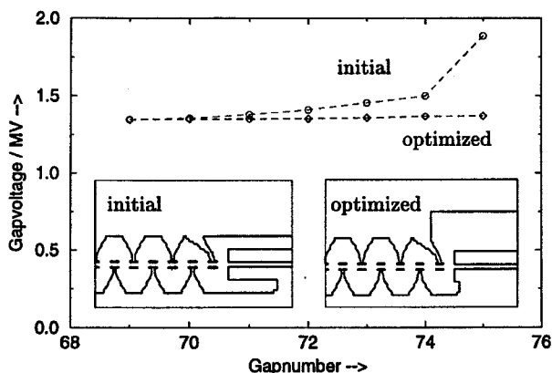
Figure 3: Optimization of the arrangement around the quadrupole lenses. The distance to the opposite girder was enlarged and the lens support was elongated.
