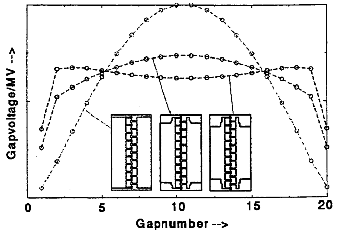
Figure 2: Voltage distribution for different depths of the undercuts in the girders.
