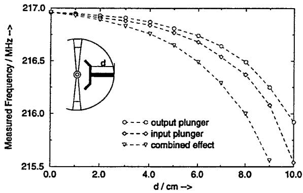
Figure 6: The LC-plunger and its effect on the resonance frequency.
