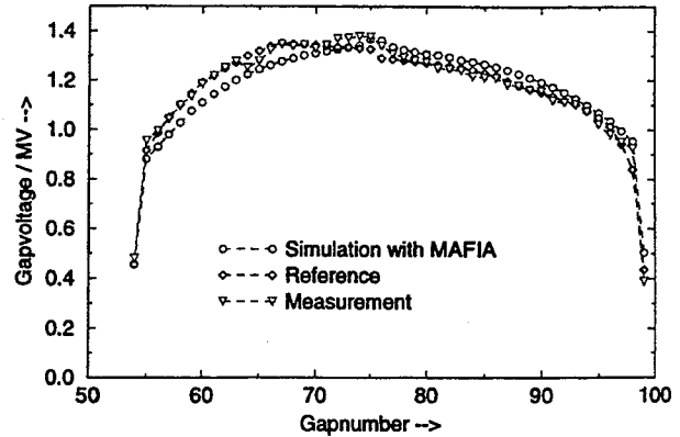
Figure 8: Calculated, measured and reference voltage distributions in cavity IH2.
