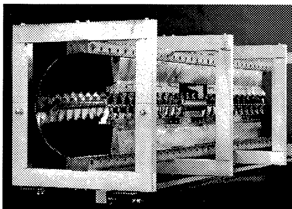
Figure 5: The 1:5.88 model for cavity IH2 (Photo: A. Zschau, GSI).
