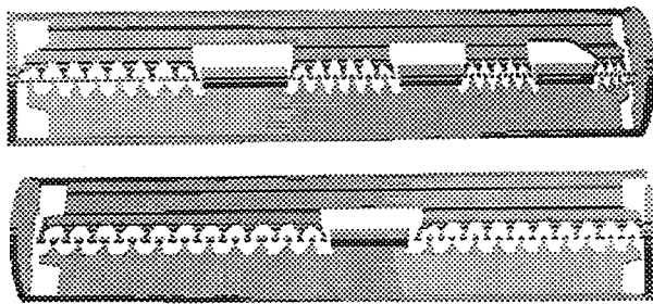
Figure 1: Layout of IH1 and IH2 after the optimization with MAFIA.
