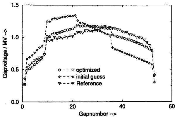
Figure 7: Calculated and reference voltage distributions in cavity IH1.
