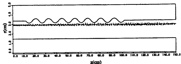
Fig. 4. Particle-in-cell simulation of coaxial geometry showing electron beam with strong axial bunching.
