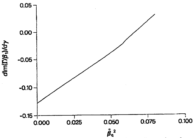
Fig. 1. Sensitivity of phase to beam energy for medium gain and low energy ( \gamma = 2 ) as a function of space charge wavenumber.
