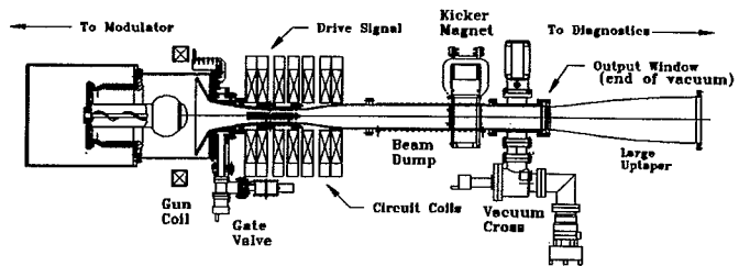
Fig. 1. The gyrokystron test bed.
