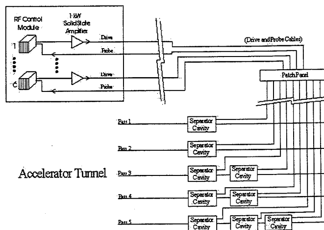
Fig. 2: RF Separator System.
