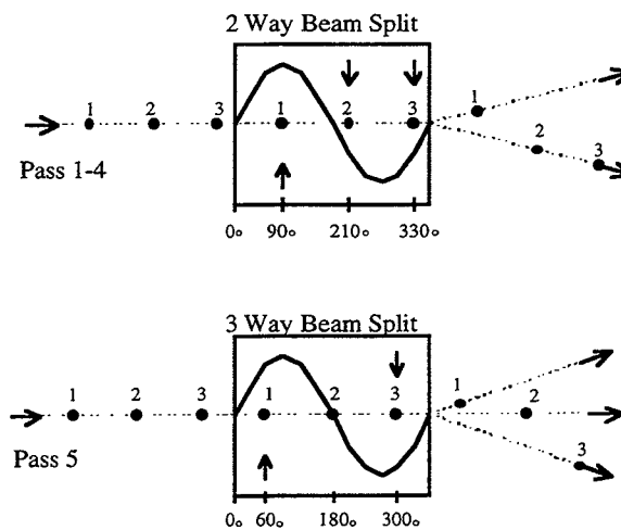
Fig. 1: Separator Cavity Phasing.
