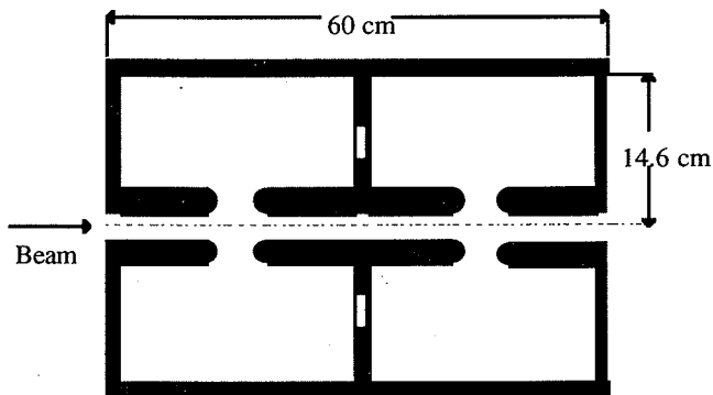
Fig. 3: Two Cell Separator Cavity.
