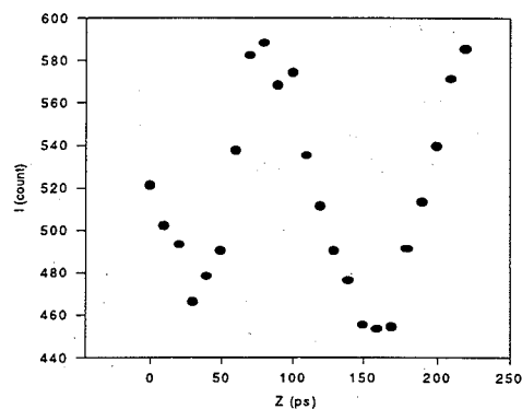
Figure 4. Measured longitudinal wakefield for the 7 GHz dielectric wakefield structure. The peak corresponds to 1.5 MV/m.
