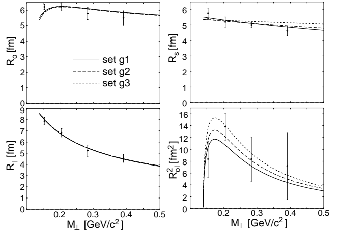
FIG. 10. Same as Fig. 9 but for the Gaussian transverse density profile with parameter sets g1, g2, g3.
