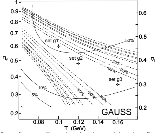
FIG. 6. Same as Fig. 5 but for the model with a Gaussian transverse density profile.
