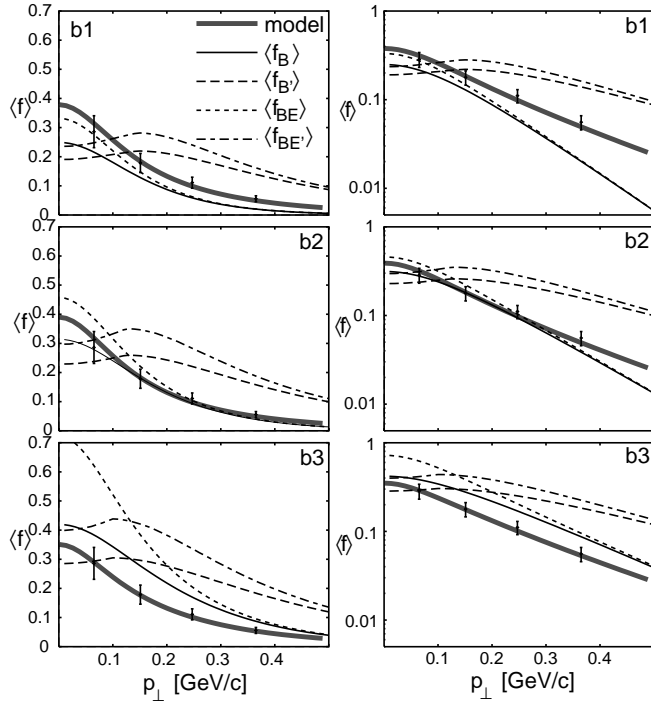
FIG. 13. Average phase-space density \langle f \rangle(\mathbf{p}) in the rapidity bin 3.9 < Y < 4.4 as a function of p_\perp . The data points are determined from NA49 data (Sec. VB1). Black lines denote expectations from the statistical treatment in Sec. VB2: \langle f_B \rangle (eq. (5.17), solid); \langle f_{B'} \rangle (eq. (5.19), long-dashed); \langle f_{BE} \rangle (eq. (5.18), short-dashed); and \langle f_{BE'} \rangle (eq. (5.20), dash-dotted). Results of our model (see text) are shown by thick solid gray lines. The symbols in the upper right corners indicate the used set of model parameters; the corresponding pionic chemical potentials are listed in Table V. The right column gives a logarithmic representation of the left column.
