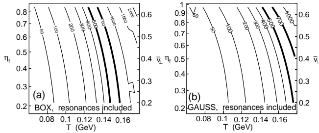
FIG. 7. Total \pi^- multiplicity (resonance decays included) as a function of T and \bar{v}_\perp , computed from the model with (a) box-shaped, (b) Gaussian transverse density profile. The wiggles in the contours towards the right in panel (a) result from numerical uncertainties in the fitted model parameters. For other details see text.
