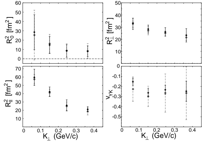
FIG. 2. The measured YKP parameters, with v_{\text{YK}} given in the LCMS. Black symbols indicate the data points from Table C2. Gray dashed symbols represent the values calculated with cross-check relations from the measured Cartesian parameters given in Table C2.
