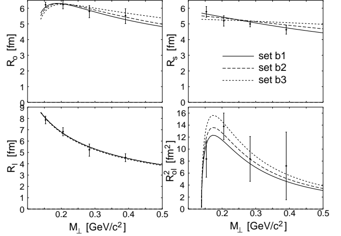
FIG. 9. Comparison of model predictions from the model with box-shaped transverse geometric profile and inserted parameter sets b1, b2, b3 with the data on Cartesian correlation radii (to which the model was fitted).
