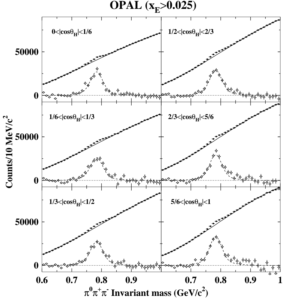
Figure 4: Invariant mass distributions of \pi^+\pi^-\pi^0 combinations for the range x_E > 0.025 , for the six equal bins of |\cos\theta_H| between 0 and 1. The black circles are the data. The full lines are the background obtained in the fits to the data. The white circles show the \omega signal, scaled by a factor 10, obtained by subtracting the fitted background (full lines) from the data. The dashed lines are the fitted signals scaled by the same factor.
