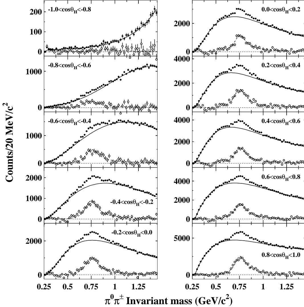
Figure 1: Invariant mass distributions of \pi^\pm\pi^0 combinations for the range 0.10 < x_E < 0.15 , for the ten equal bins of \cos\theta_H between -1 and +1 . The black circles are the data. The full lines are the background obtained in the fits to the data. The white circles show the \rho^\pm signal, scaled by a factor 2, obtained by subtracting the fitted background (full lines) from the data. The dashed lines are the fitted signals scaled by the same factor.
