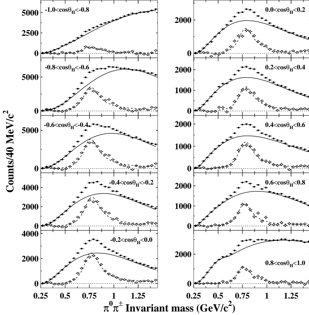
Figure 2: Invariant mass distributions of \pi^\pm \pi^0 combinations for the scaled energy range 0.3 < x_E < 0.6 , for the ten equal bins of \cos \theta_H between -1 and +1 . The black circles are the data. The full lines are the background obtained in the fits to the data. The white circles show the \rho^\pm signal, scaled by a factor 2, obtained by subtracting the fitted background (full lines) from the data. The dashed lines are the fitted signals scaled by the same factor.
