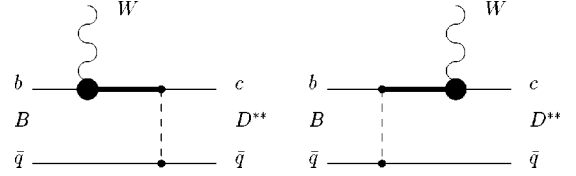
FIG. 2. Vertex function \Gamma^{(2)} taking the quark interaction into account. Dashed lines correspond to the effective potential (12). Bold lines denote the negative-energy part of the quark propagator.
