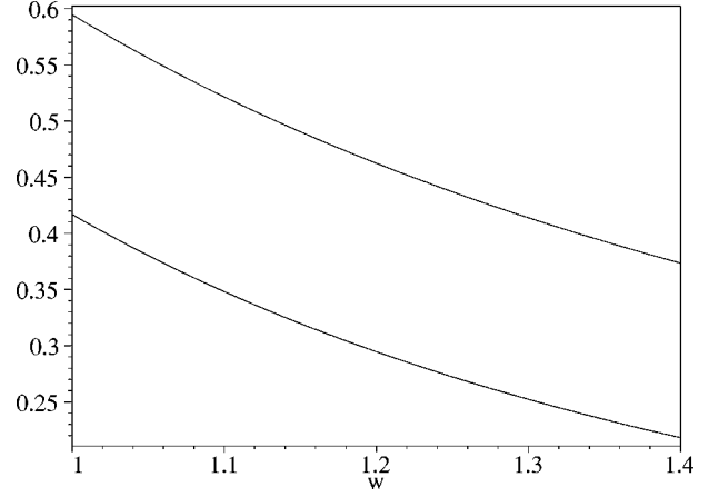
FIG. 4. Isgur-Wise functions \zeta(w) (upper curve) and \zeta_1(w) (lower curve) for the B \rightarrow D_{0,1}^* e \nu decay.
