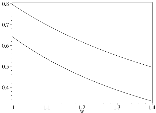
FIG. 6. Isgur-Wise functions \zeta(w) (upper curve) and \zeta_1(w) (lower curve) for the B_s \rightarrow D_{s,0,1}^* e \nu decay.
