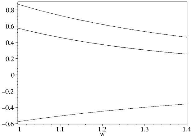
FIG. 3. Isgur-Wise functions \tau(w) (upper curve), \tau_1(w) (middle curve), and \tau_2(w) (lower curve) for the B \rightarrow D_{1,2} e \nu decay.
