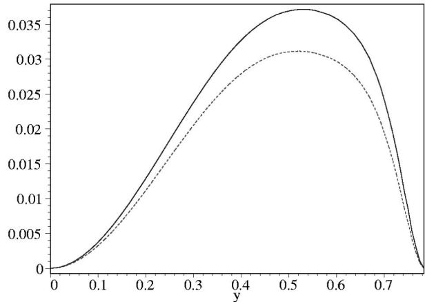
FIG. 7. Electron spectra (1/\Gamma_0)(d\Gamma/dy) for the B \rightarrow D^{**} e \nu decays. Dashed curves show the m_Q \rightarrow \infty limit, solid curves include first-order 1/m_Q corrections.
