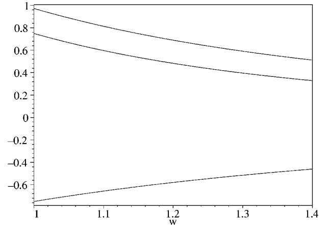
FIG. 5. Isgur-Wise functions \tau(w) (upper curve), \tau_1(w) (middle curve), and \tau_2(w) (lower curve) for the B_s \rightarrow D_{s,1,2} e \nu decay.
