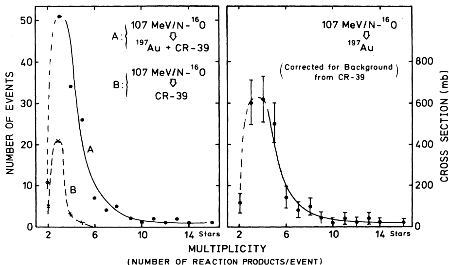
FIG. 3. Cross sections for the production of events of different multiplicities in the interaction of 107 MeV/N ^{16}\text{O} ions with ^{197}\text{Au} .
