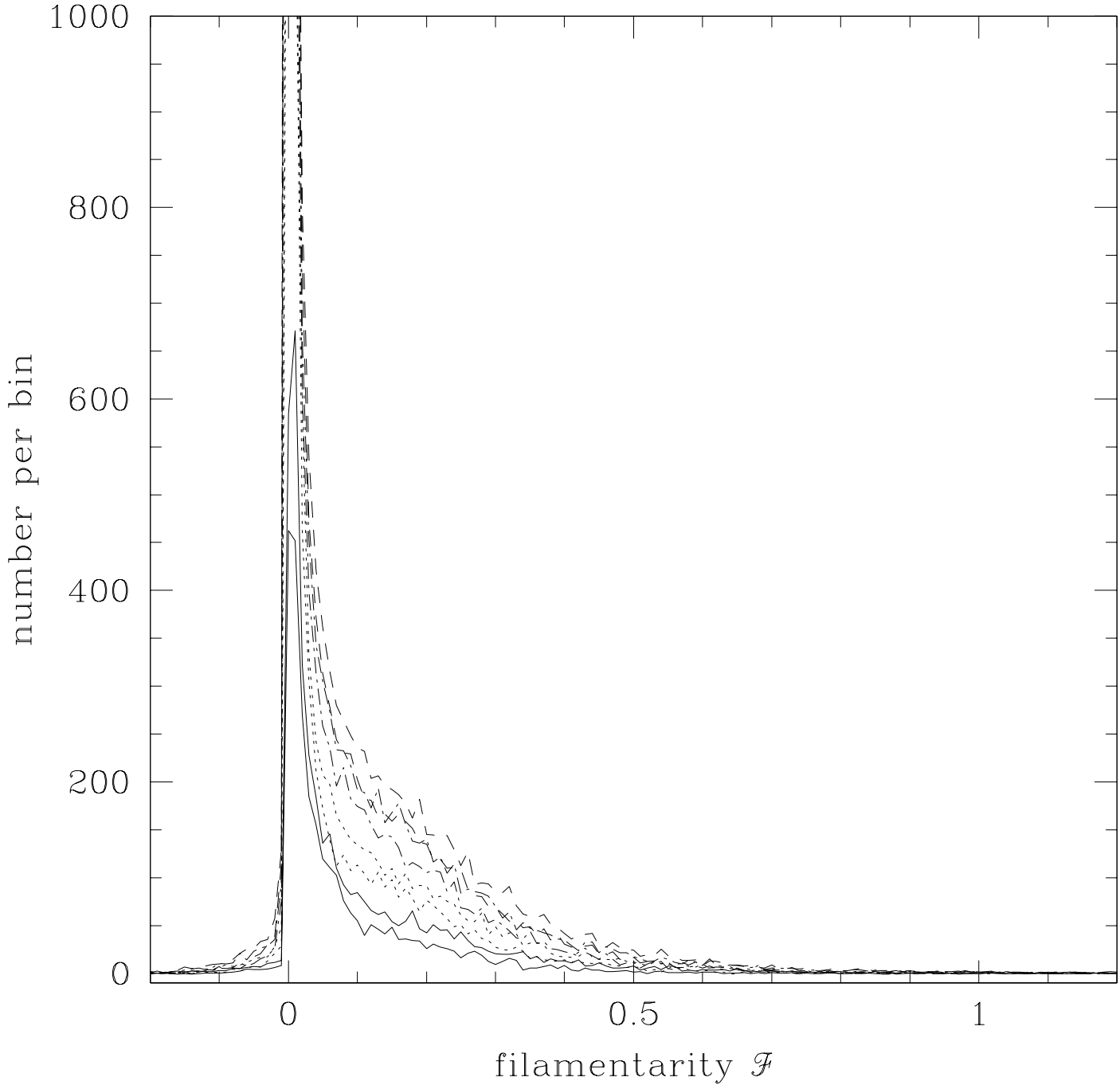
Fig. 12.— This figure displays the same type of distribution as above, but shows the filamentarity shapefinder \mathcal{F} . Line styles are explained in Figure 2.
