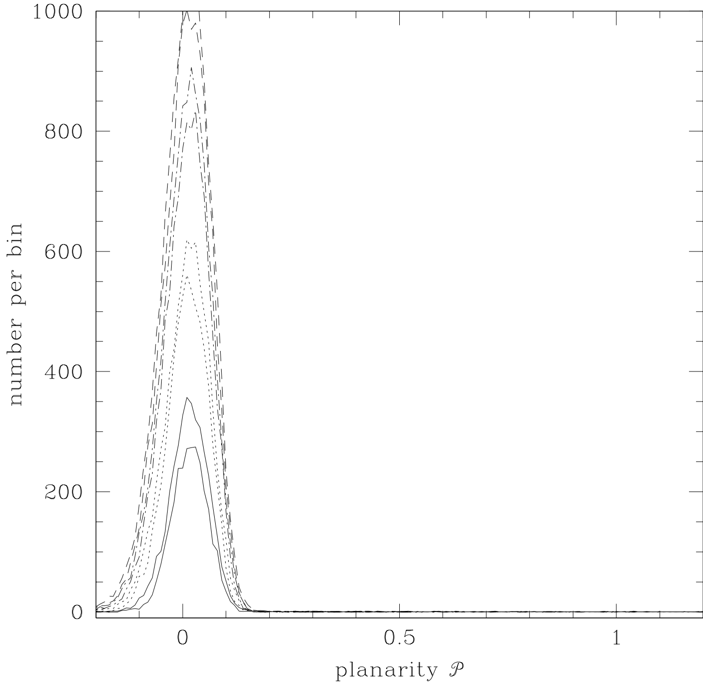
Fig. 11.— The distribution of the planarity shapefinder \mathcal{P} . The histogram only includes objects larger than 10^{-5} times the simulation box, a value of the order of the smoothing volume. Note that although theoretically, the value should lie between 0 and 1, measurement
