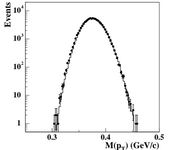
FIG. 1. Event-by-event distribution of the mean transverse momentum M(p_T) of accepted particles in the event (points). For comparison, the solid line shows the M(p_T) distribution for mixed events.
