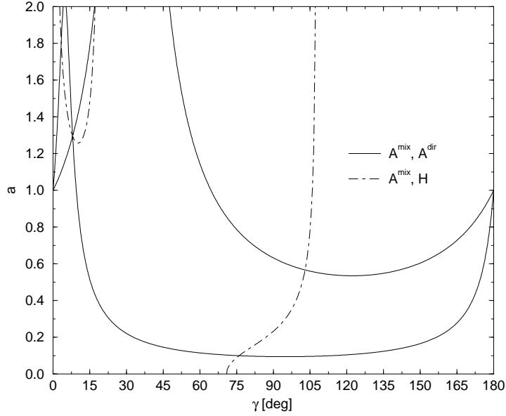
Figure 4: The contours in the \gamma-\tilde{a} plane fixed through the B_{d(s)} \rightarrow D_{d(s)}^+ D_{d(s)}^- observables for a specific example discussed in the text ( 2\beta = 53^\circ ).
