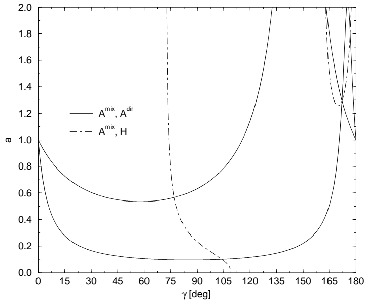
Figure 5: The contours in the \gamma-\tilde{a} plane fixed through the B_{d(s)} \rightarrow D_{d(s)}^+ D_{d(s)}^- observables for a specific example discussed in the text ( 2\beta = 180^\circ - 53^\circ ).
