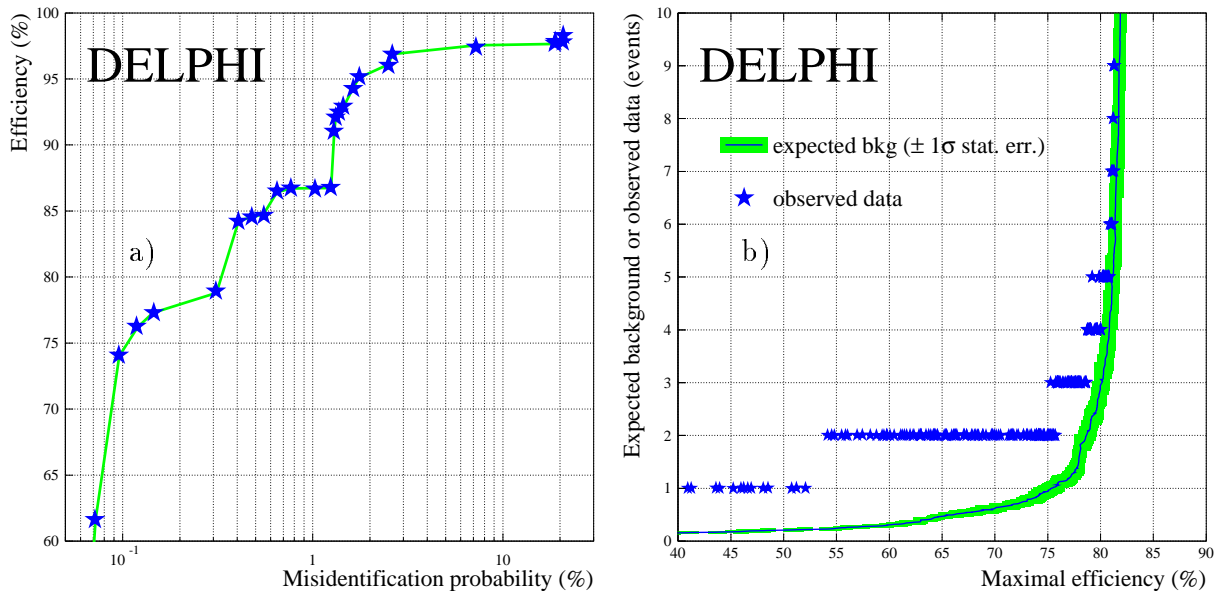
Figure 2: H\mu^+\mu^- channel: a) the performance of the muon identification. Efficiency is given for muons with momentum above 10 \text{ GeV}/c coming from Z \rightarrow \mu^+\mu^-(\gamma) events at 183 \text{ GeV} . The probability of misidentifying a charged hadron as a muon is measured using charged kaons and pions coming from Z \rightarrow \tau^+\tau^-(\gamma) events. The kinks correspond to changes in the way the information is combined. b) Expected background as a function of the maximal efficiency obtained at each background level for a Higgs signal of m_H = 85 \text{ GeV}/c^2 . Statistical errors are indicated by the narrow band around the curve. Stars correspond to the number of observed data events for a given working point. Notice that the working point definition involves optimizing several cuts simultaneously, and not a cut on just one variable. Thus the events selected at any given efficiency need not be a subset of those at higher efficiencies, and this explains the overlap when 4 or 5 events are observed.
