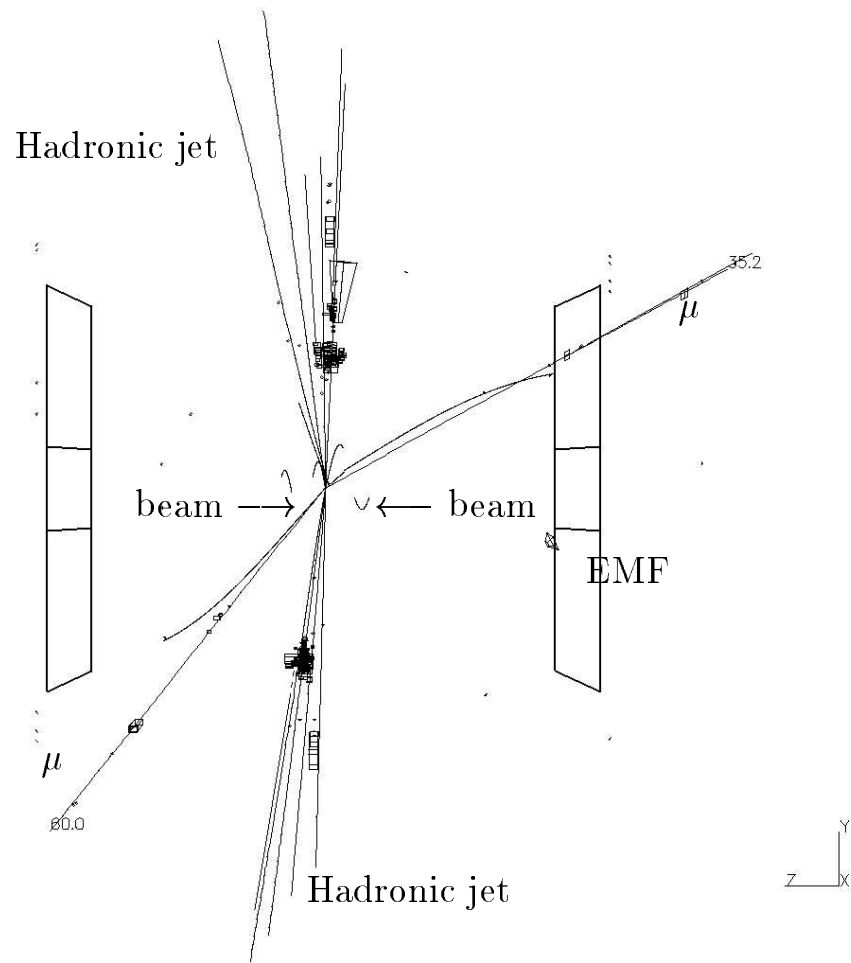
Figure 4: H\mu^+\mu^- channel: longitudinal view of the event with little evidence for b quarks. The reconstructed charged particle tracks, energy deposits and the geometry of the forward electromagnetic calorimeters (EMF) are displayed. The two muon candidates are the tracks isolated from the jets.
